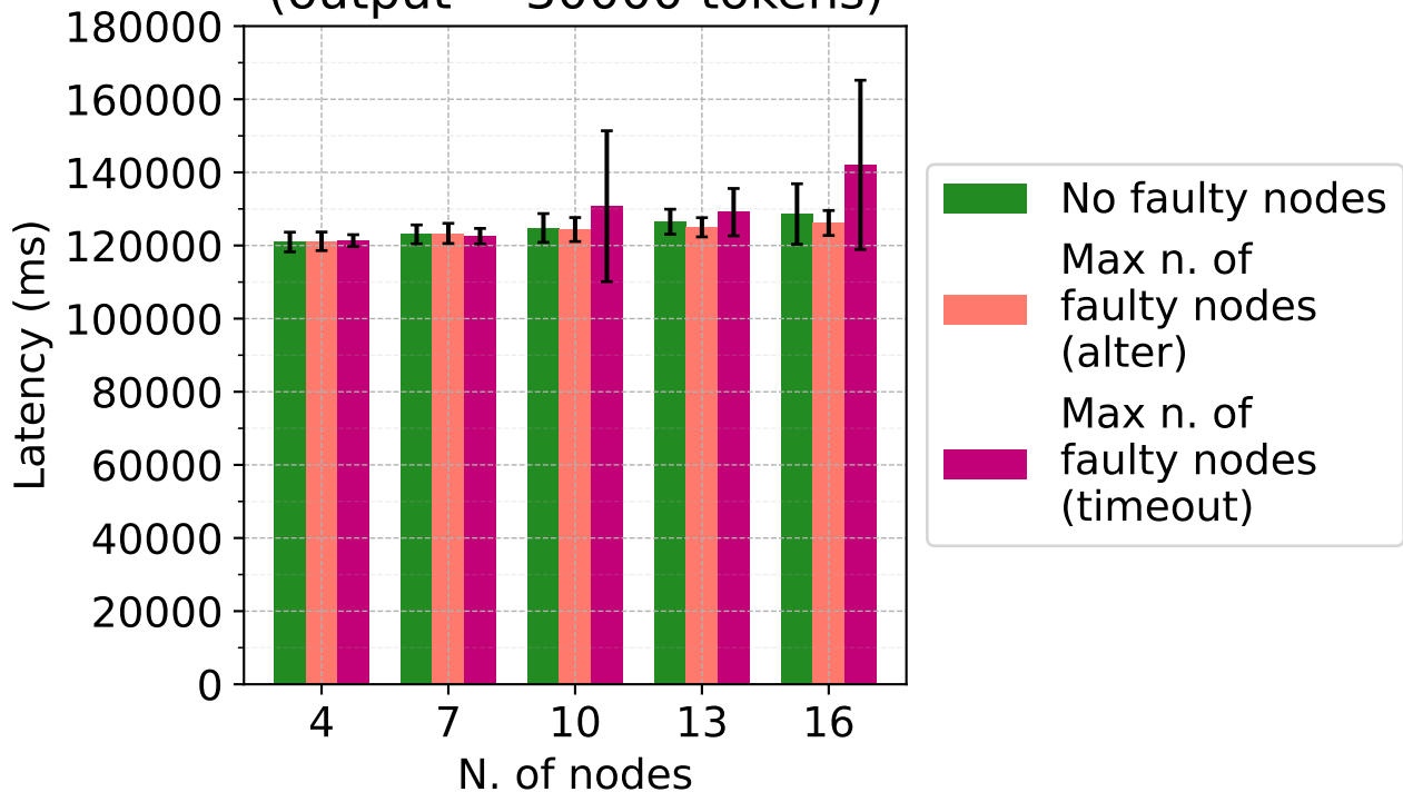
Total latency (output = 30000 tokens)
