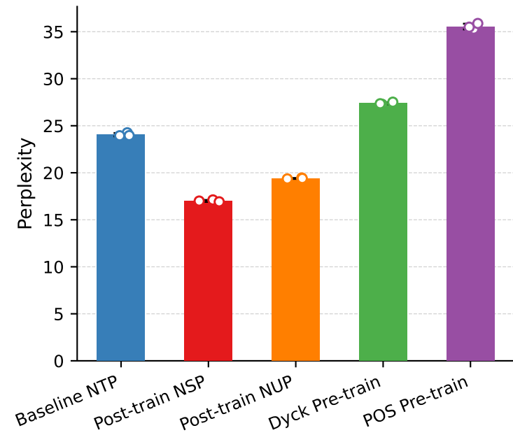
10M tokens
