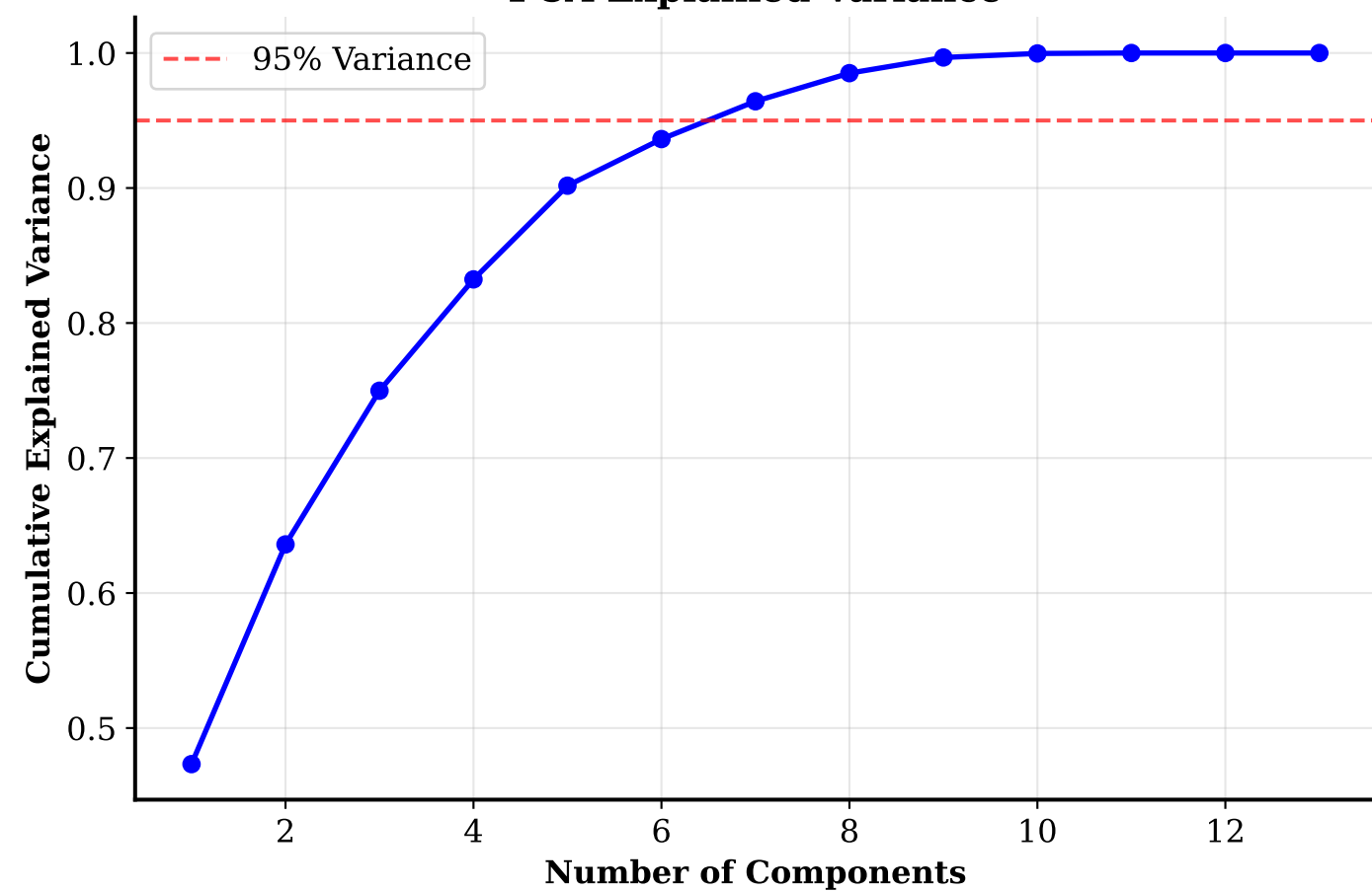
PCA Explained Variance
