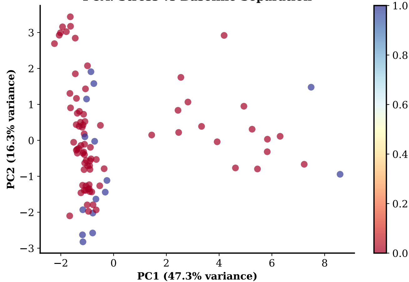
PCA: Stress vs Baseline Separation
