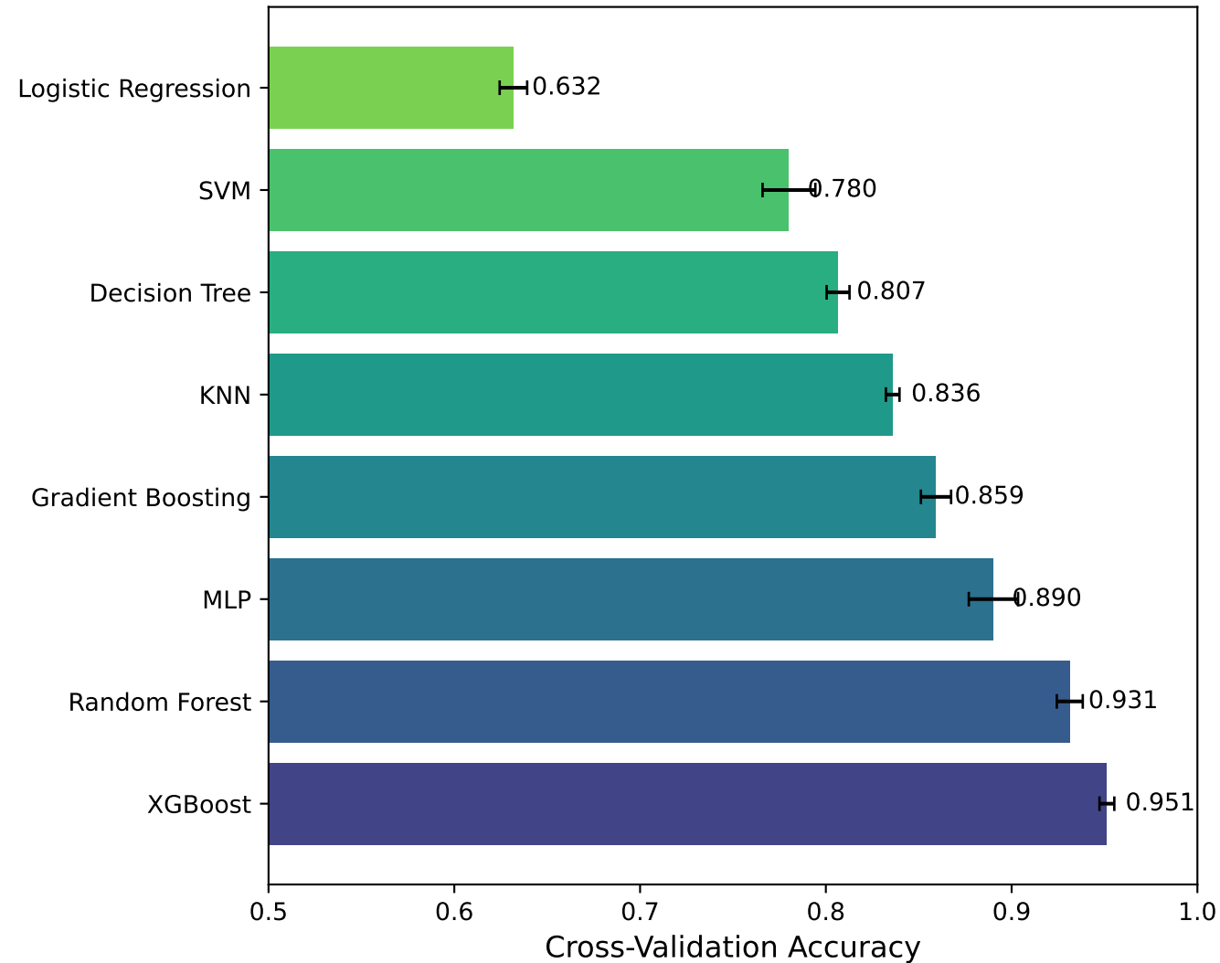
Model Comparison: CV Accuracy
