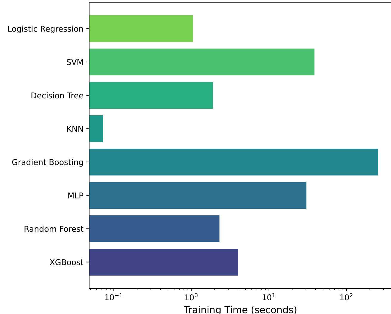
Model Comparison: Training Time
