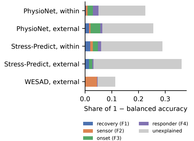
Fig. 4. Error budget. Each bar is 1–BA of the out-of-sample predictions; coloured segments are the Shapley-averaged gains of the four test-side filters, grey is the residual after all four. Negative gains (Stress-Predict external, F2) are drawn as zero.
