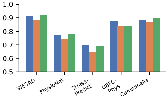
Balanced accuracy (held-out subjects)
