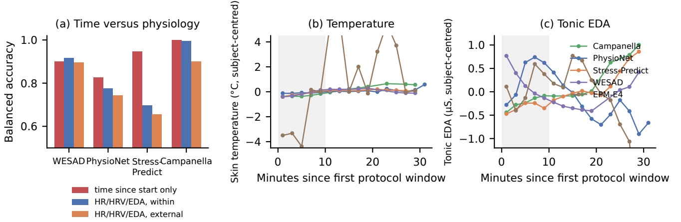
Fig. 3. (a) Balanced accuracy of a classifier that sees only minutes since recording start, against the HR/HRV/EDA model within and across datasets. (b), (c) Subject-centred skin temperature and tonic EDA against minutes since the first protocol window (2-min bins); the shaded band marks the first 10 min, in which 100% of Campanella, 97% of Stress-Predict and 68% of PhysioNet baseline windows fall when measured from recording start (90% within 15 min). WESAD’s protocol clock starts 16–26 min after its recording; EPM-E4’s starts at recording.
