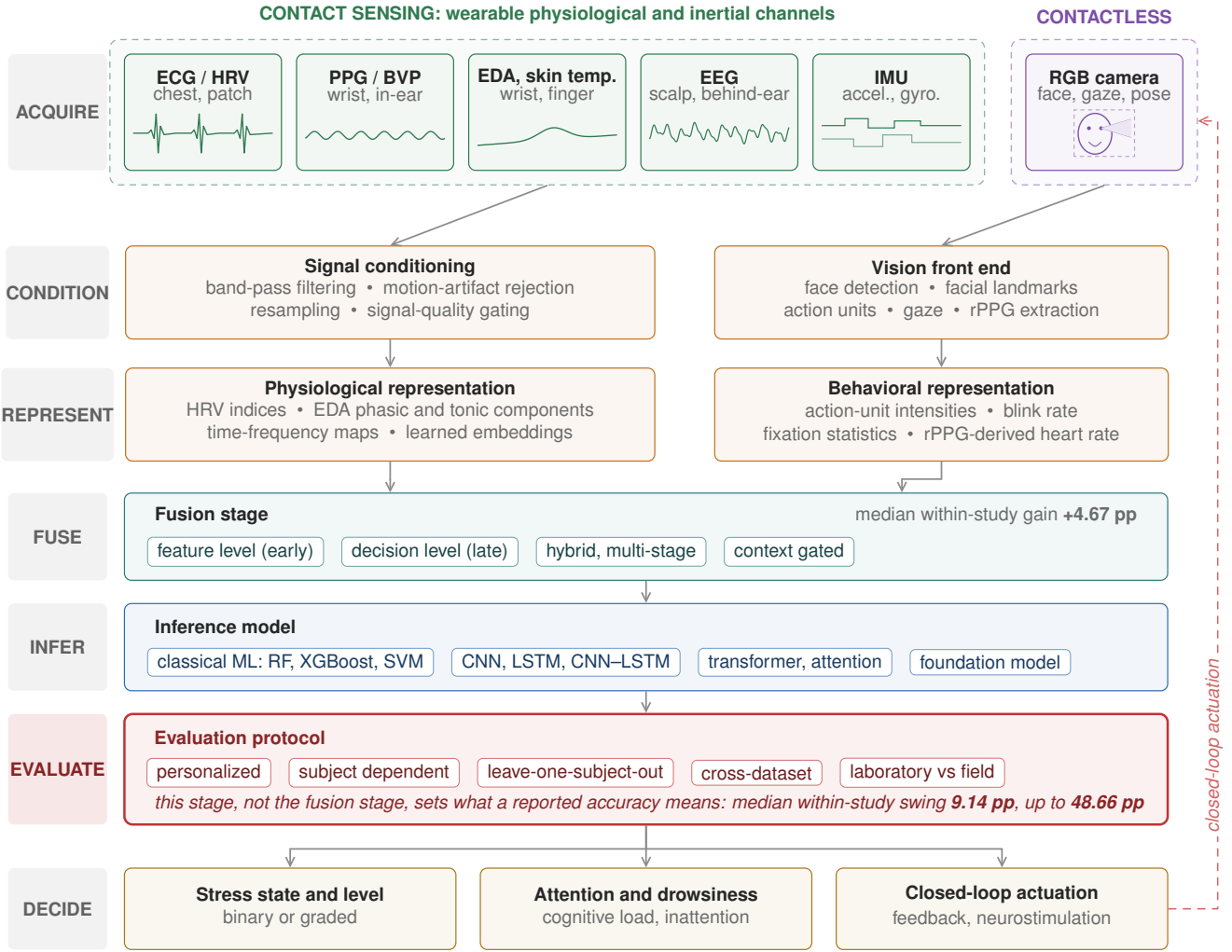
Figure 1: Seven-stage processing chain shared by the wearable and camera-based stress and attention monitoring systems reviewed here, with a representative trace drawn inside each acquisition card. Contact channels (green) and the contactless camera channel (purple) are conditioned and represented separately before being combined at a feature, decision, hybrid or context-gated fusion stage and passed to an inference model. The evaluation protocol is drawn as a stage of equal standing, and highlighted, because it is the stage that determines what a reported accuracy means: the median within-study swing attributable to it is 9.14 percentage points against 4.67 for the fusion stage. The dashed return path denotes closed-loop actuation, in which a decision drives stimulation or feedback that the sensors then observe.
