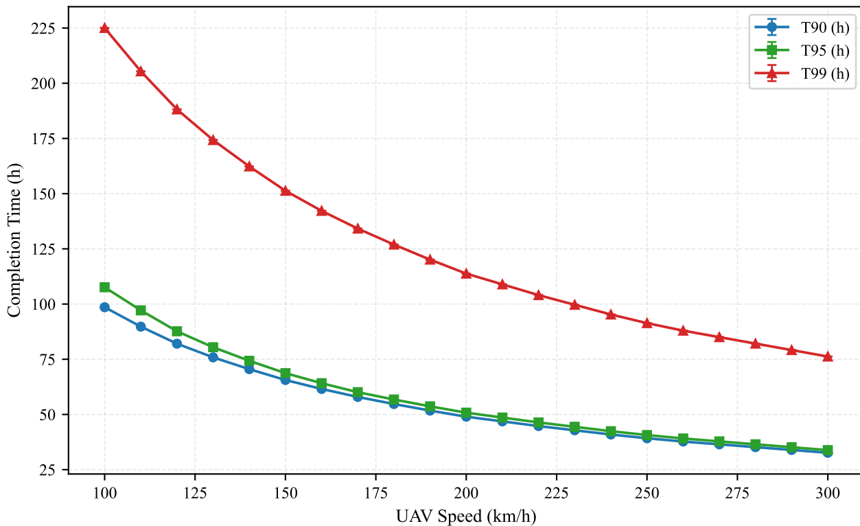
Figure 16 Completion Time vs UAV Speed (Single UAV, Non-Dynamic)
