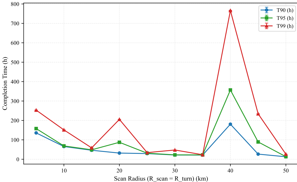
Figure 17 Completion Time vs Scan Radius (Single UAV, Non-Dynamic)
