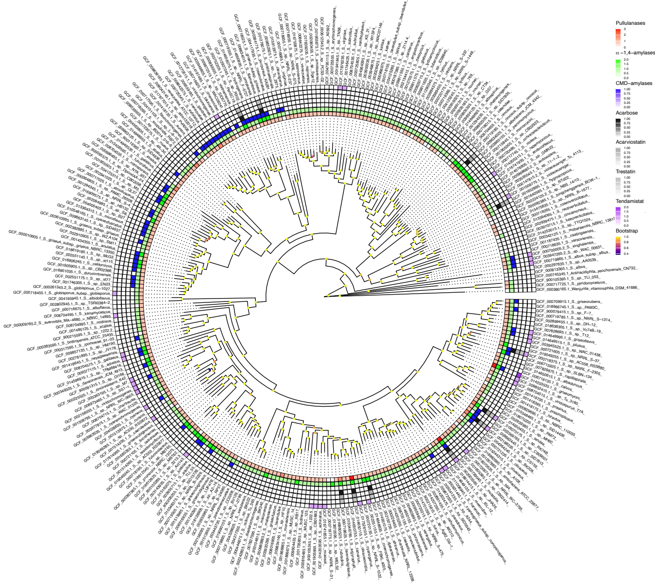
Figure 2: Amylases frequently co-occur with amylase inhibitors in Streptomyces genomes. The evolutionary relationship between 295 Streptomyces species were inferred from whole genome phylogeny and the prevalence of amylases and amylase inhibitors is visualised using a colour scale (white indicates absence; darker colours indicate higher prevalence). Annotations shown in the legend (right panel), listed from top to bottom, correspond to the concentric circles around the phylogenetic tree from the innermost to the outermost. Pullulanases (innermost, red) and \alpha -1,4-amylases (green) are found almost ubiquitously throughout the Streptomyces genus, whereas only a subset of species encode cyclomaltodextrin-like amylases (blue). Genomes with higher numbers of amylases frequently coincide with those encoding amylase inhibitors, including acarbose (black), acarviostatin (darkgrey), trestatin (grey), and tendamistat (purple). Branch support values (Bootstrap), computed as Transfer Bootstrap Expectation scores, are represented by coloured circles at internal nodes.
