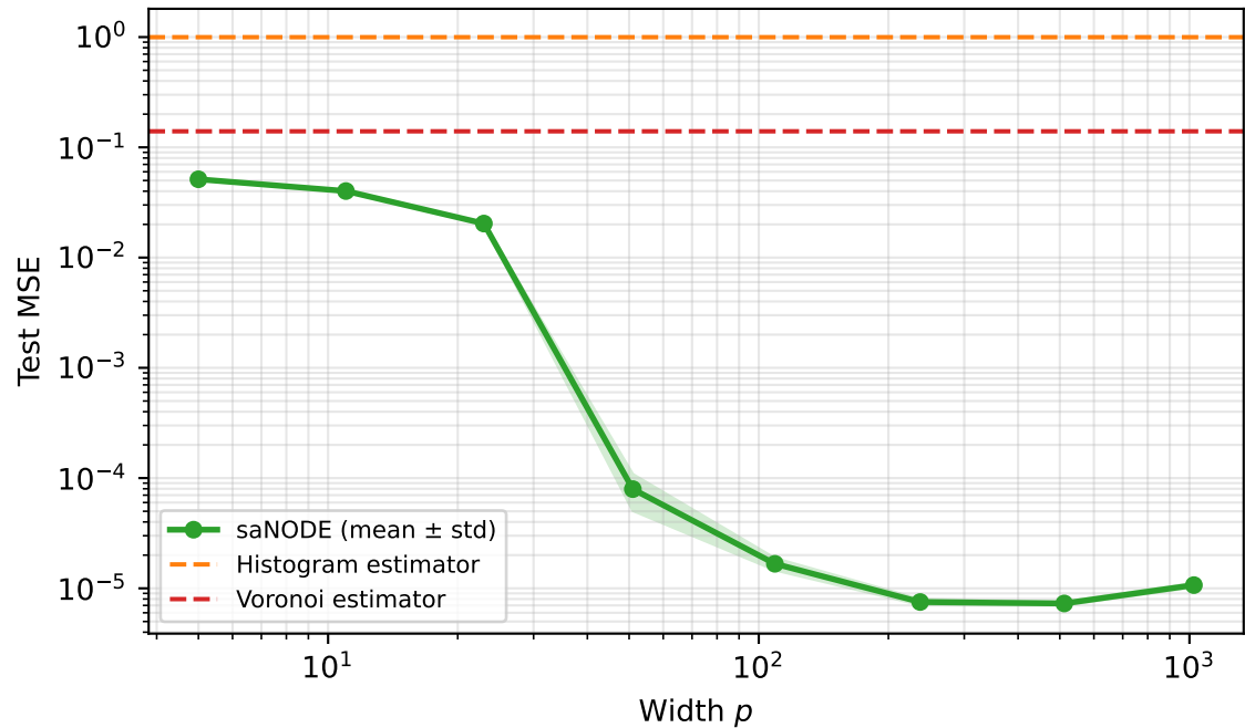
Hölder-1/2 target, N = 5000 , d = 8
