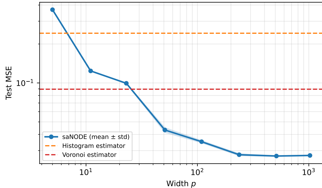
Smooth target, N = 5000 , d = 8
