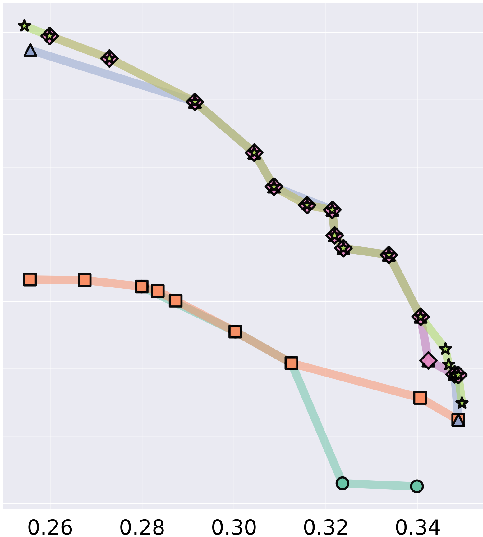
Certified Accuracy
