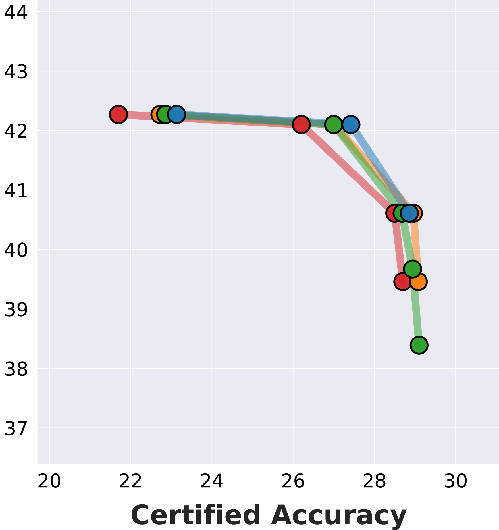
Natural Accuracy
