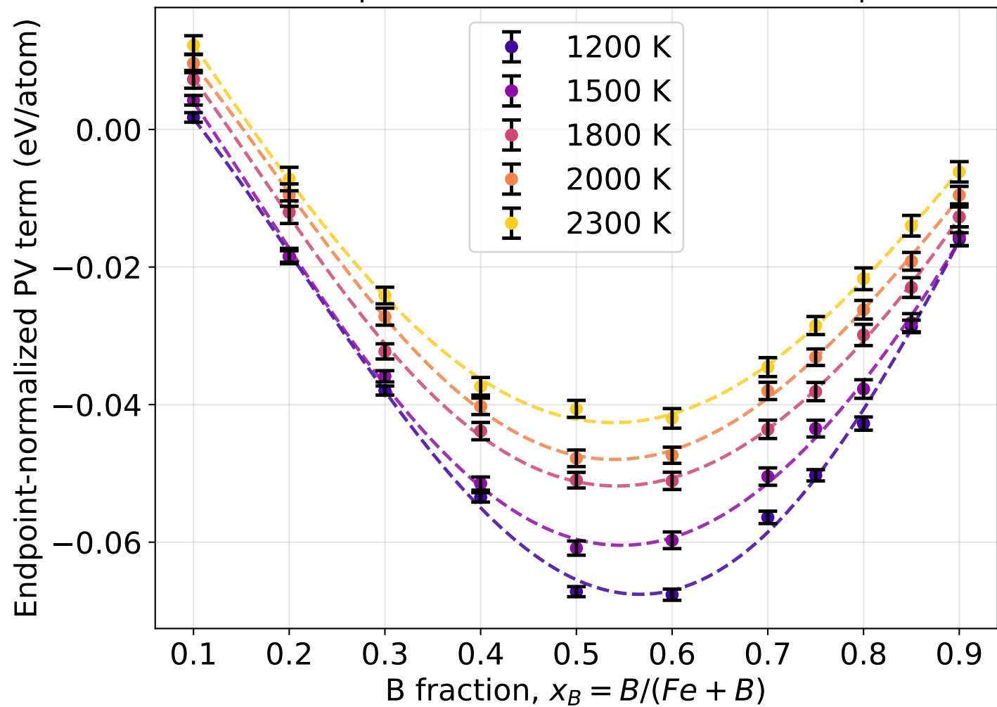
10 GPa: endpoint-normalized PV term vs composition
