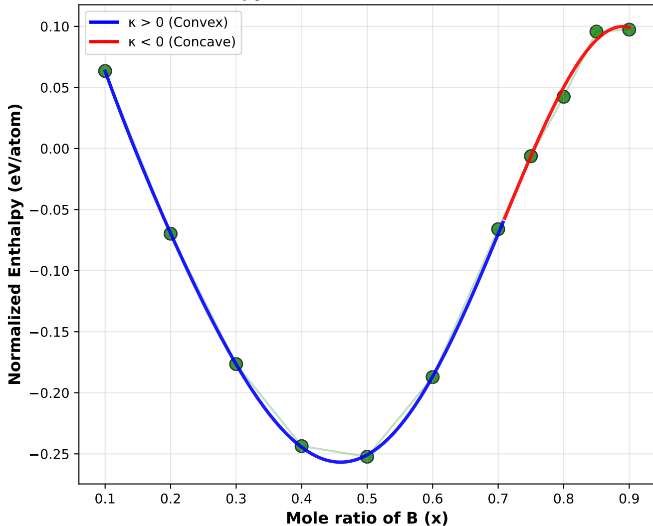
Enthalpy vs x(B) at 1500 K and 10 GPa
