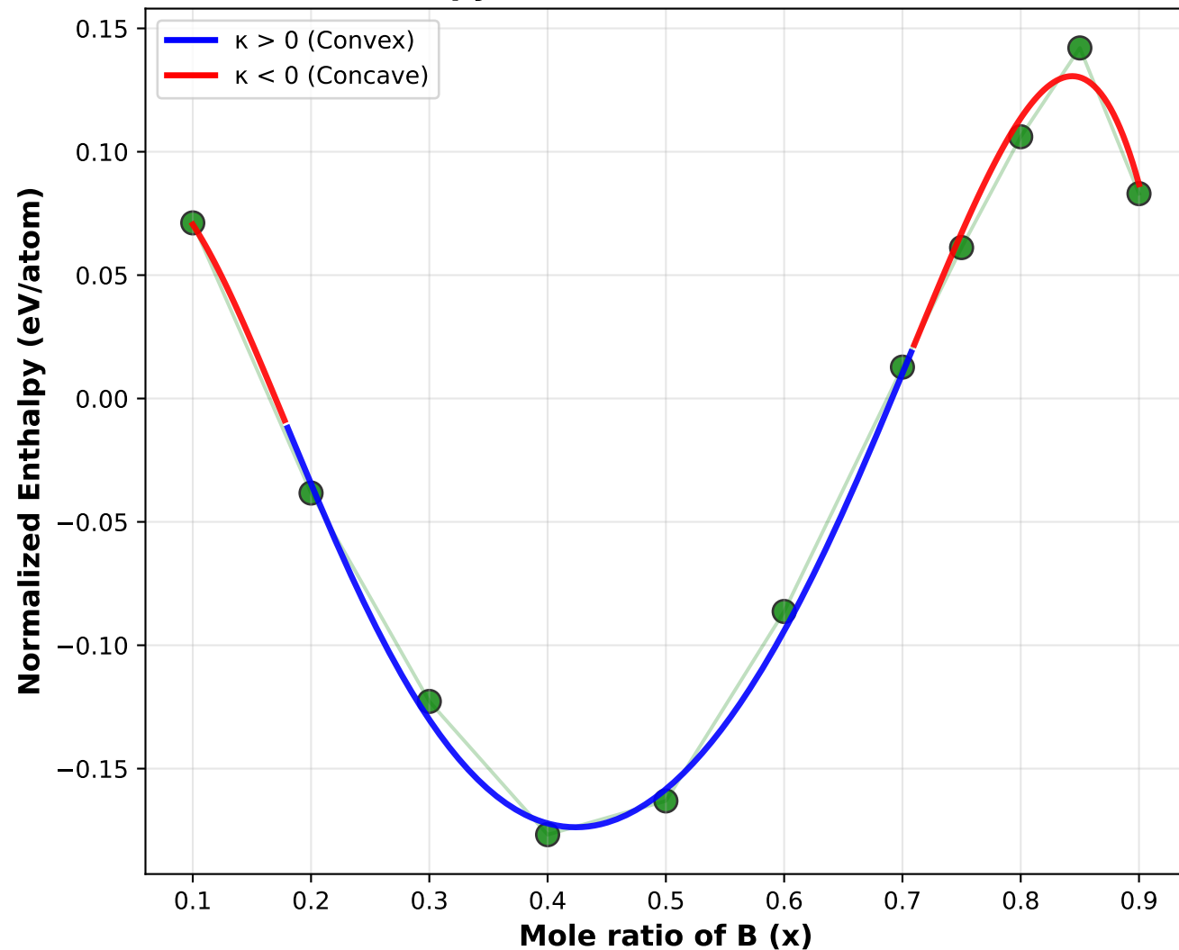
Enthalpy vs x(B) at 1500 K and 0 GPa
