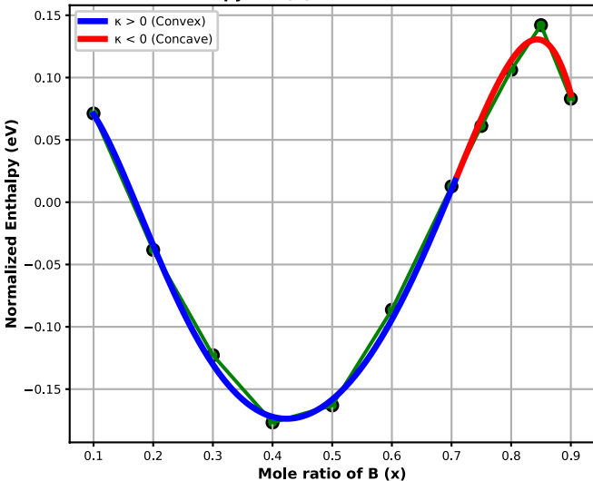
Enthalpy vs x(B) at 1500 K and 0 GPa
