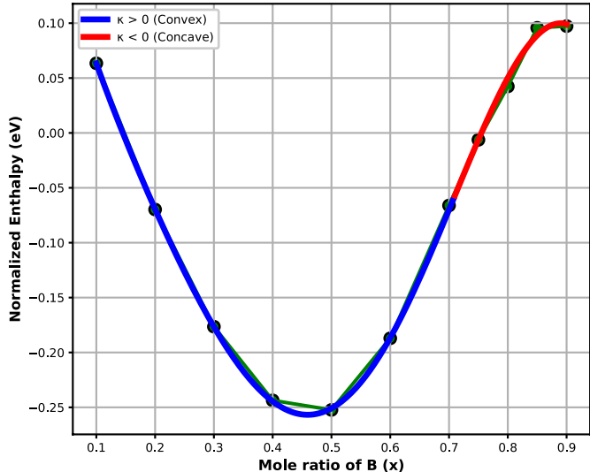
Enthalpy vs x(B) at 1500 K and 10 GPa
