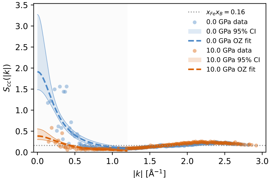
Fe-B, x_B = 0.80 , OZ fits with 95% CI
