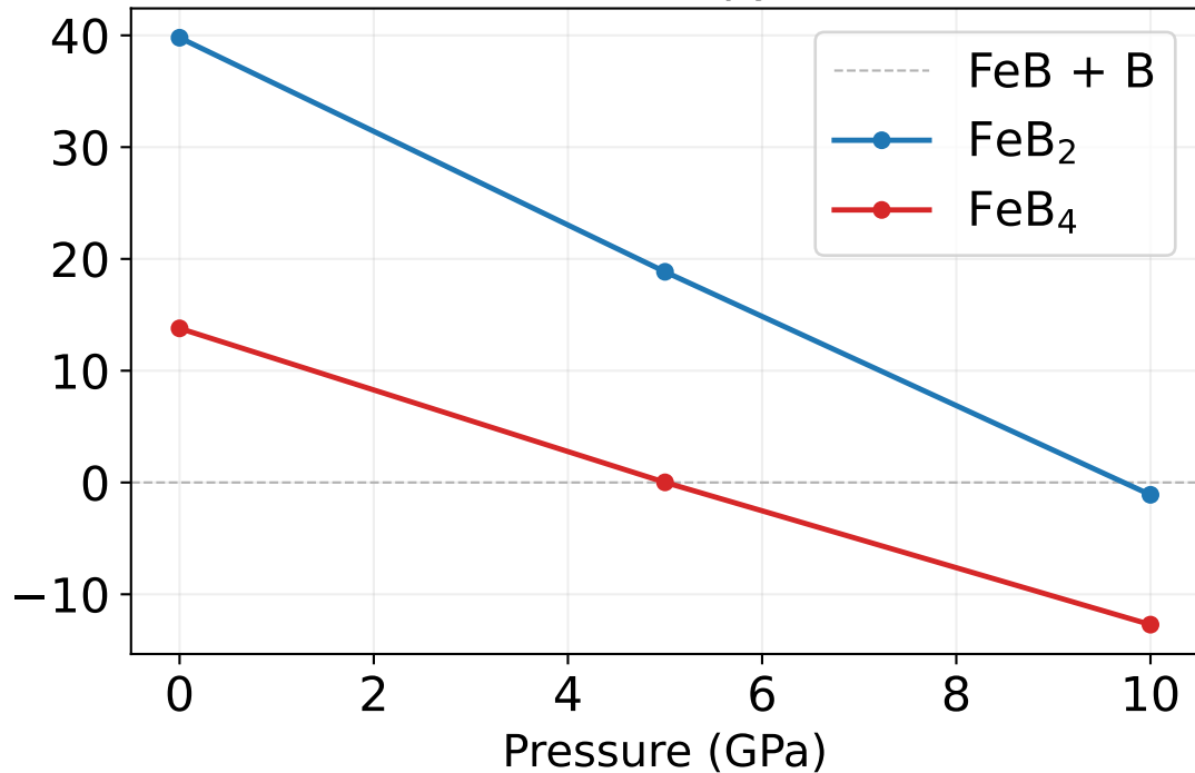
Formation enthalpy from DFT
