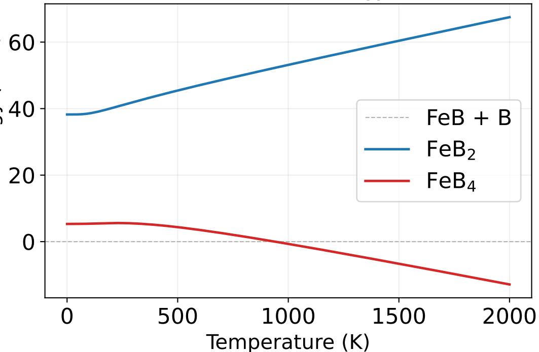
0 GPa formation free energy from DFT
