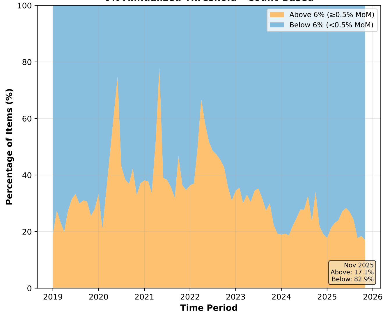
6% Annualized Threshold - Count-Based
