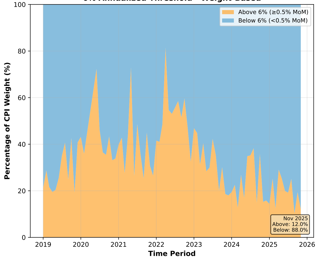
6% Annualized Threshold - Weight-Based
