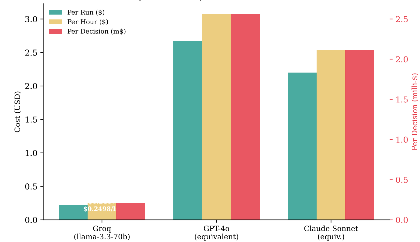
C — API Cost Estimation [Estimated | 320 tokens/decision | 1041 cycles | 70/30 in/out split] □ Groq was used locally — no actual API cost incurred
