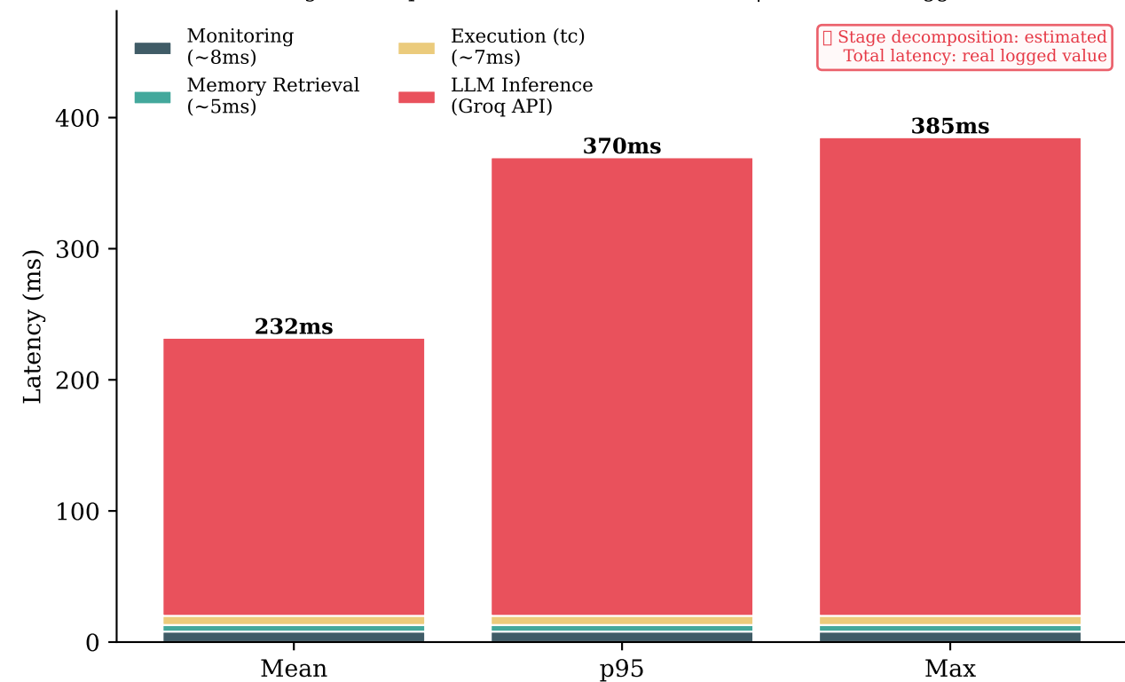
D — Decision Latency Breakdown Mean=232ms p95=370ms Max=385ms LLM share=91% [Stage decomposition: architectural estimate | Total = real logged]
