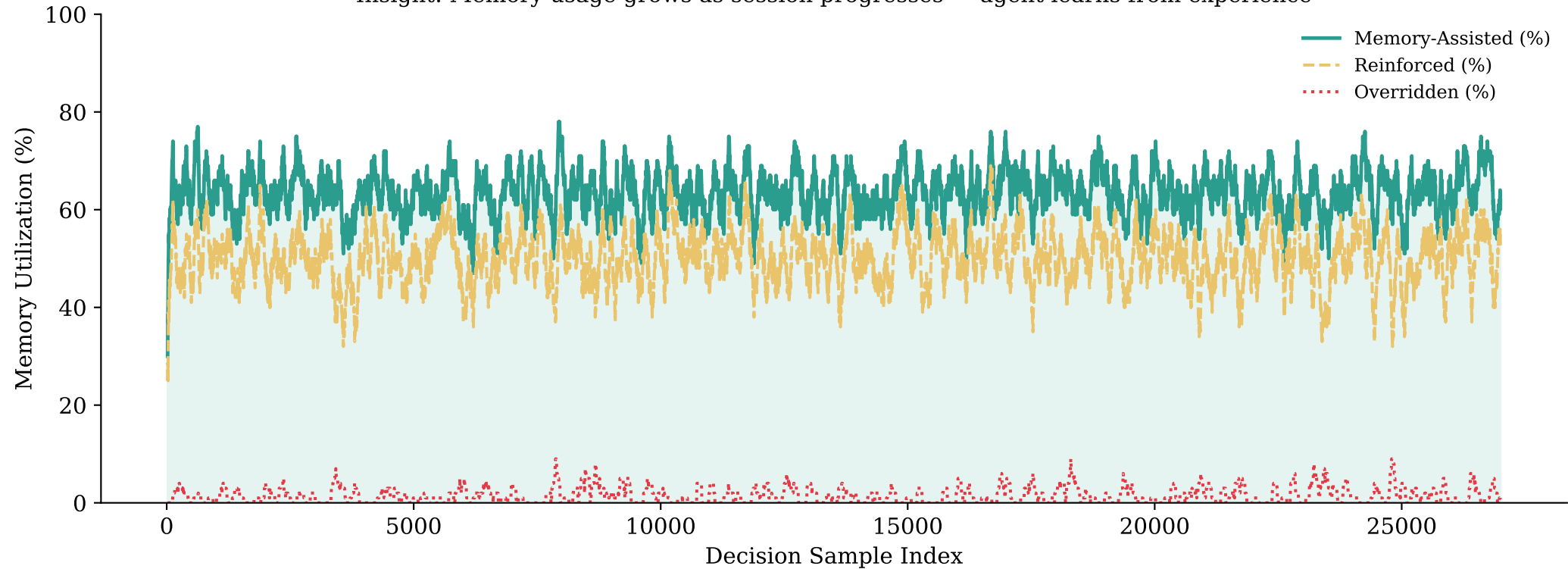
RQ4 — C5: Memory Utilization Over Time (Rolling Window=100) Insight: Memory usage grows as session progresses — agent learns from experience
