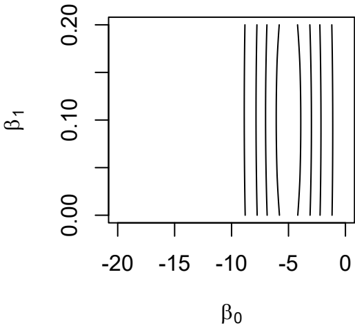
Joint Prior
