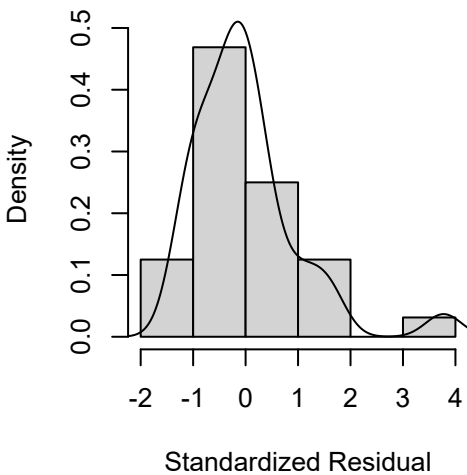
Distribution of Standardized Res.
