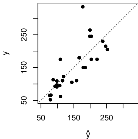
Observed vs. Fitted Values
