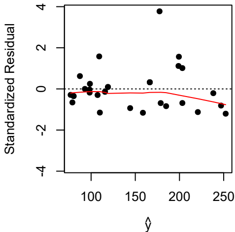
Standardized Residual vs. Fitted
