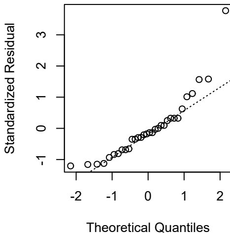
Q-Q Plot of Standardized Res.
