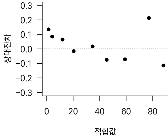
(a) OLS
