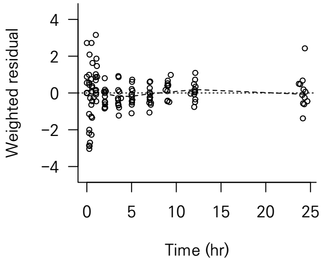
(b) CWRES (EBE 전개)
