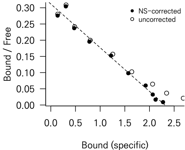
(b) Scatchard
