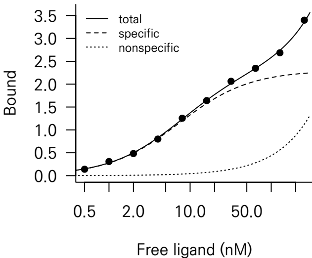
(a) saturation
