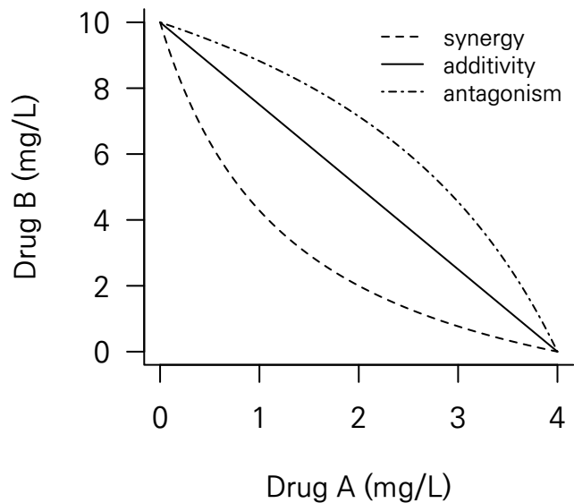
(a) isobologram
