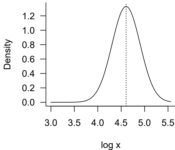
(b) Normal after taking logs
