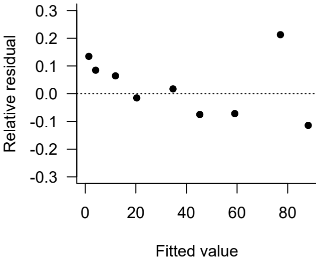
(a) OLS
