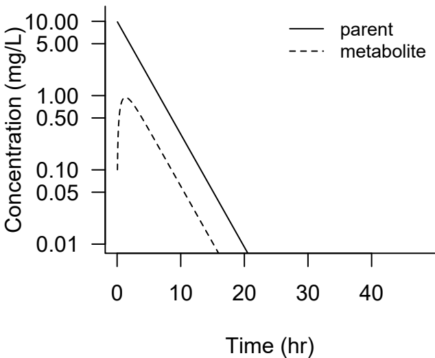
(a) formation-limited ( k_m > k_p )
