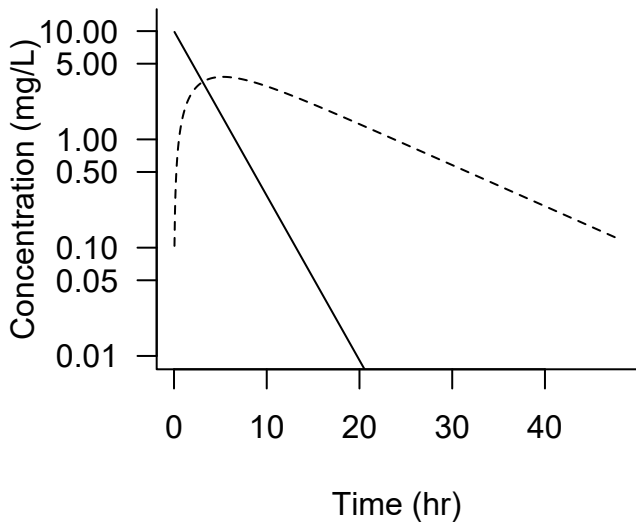
(b) elimination-limited ( k_m < k_p )
