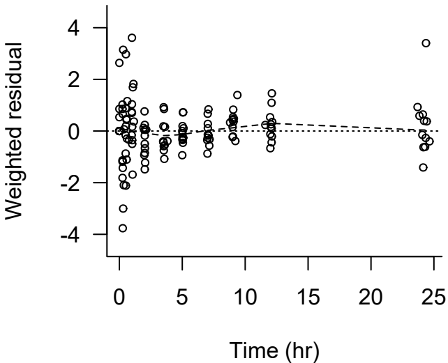
(a) WRES (expansion at \eta = 0 )
