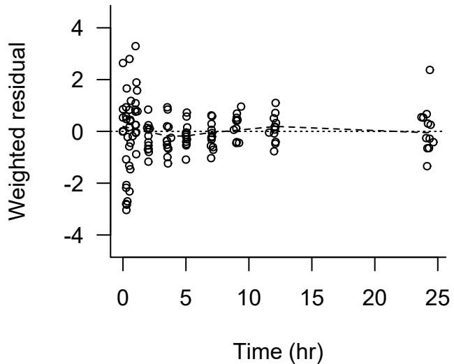
(b) CWRES (expansion at the EBE)
