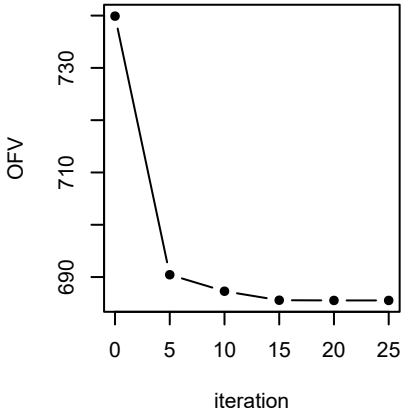
objective function
