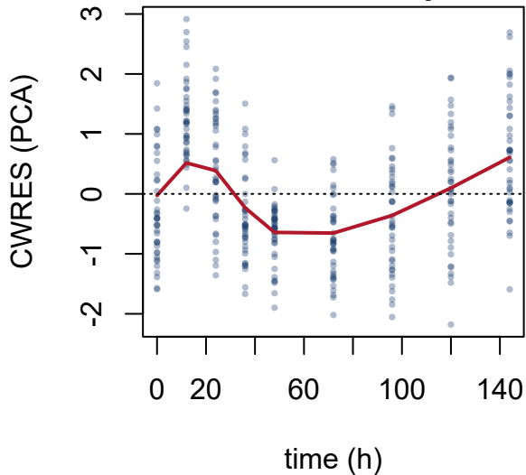
residuals of the effect-compartment
