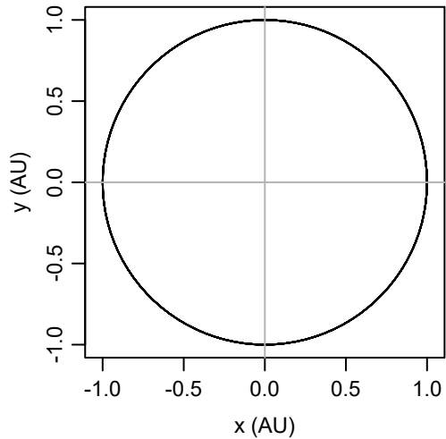
RK4
