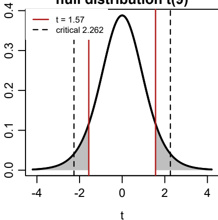
null distribution t(9)
