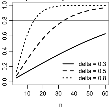
power at \alpha = 0.05
