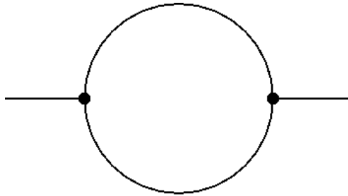
Figure1.1: Bubble (one-loop two-point) topology.
