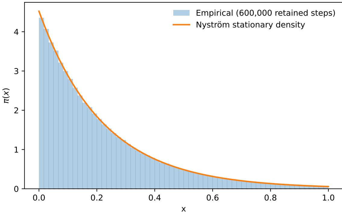
Stationary density: \beta_1 = 5 , \gamma = 2.5 , K = 1
