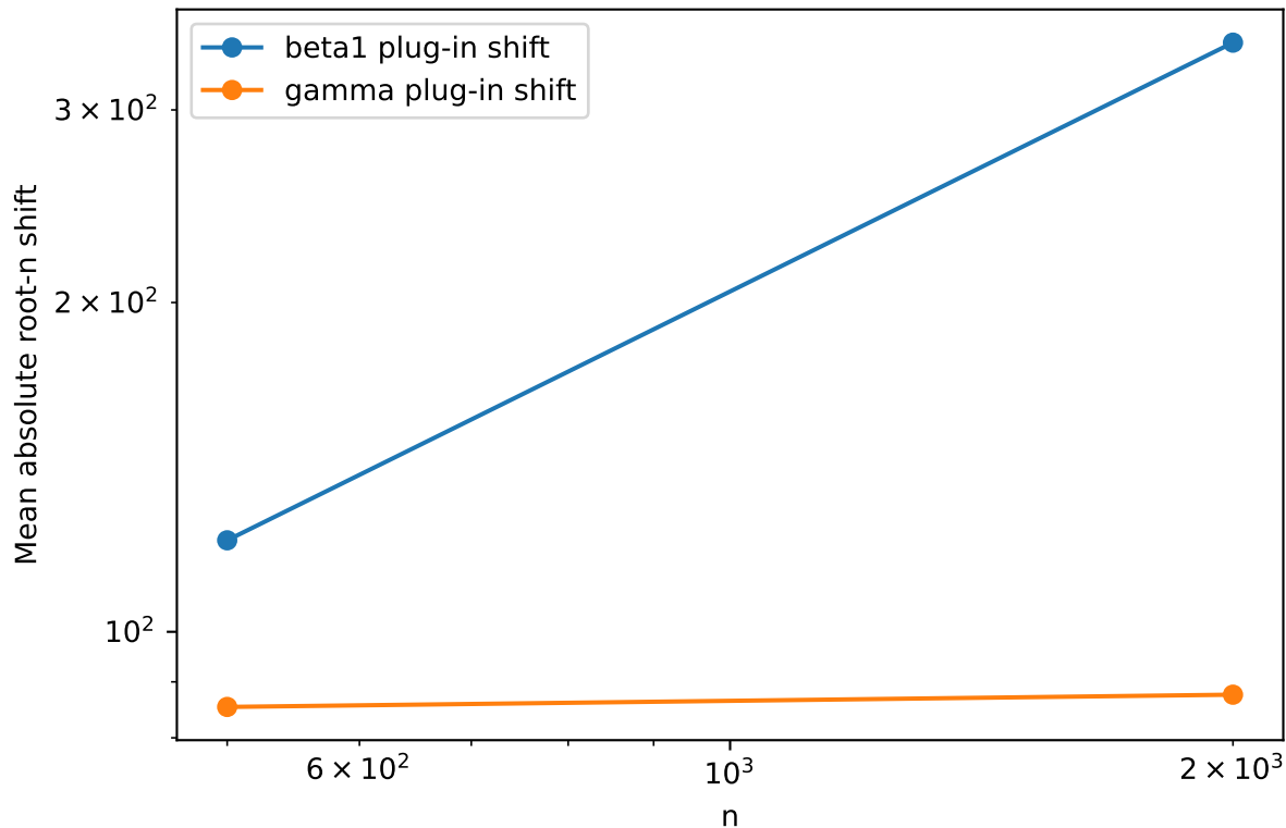
Failure outside endpoint-rate assumptions (beta AR)
