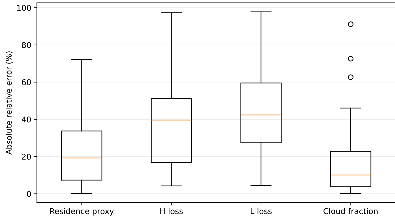
Absolute metric error at the diffusion-selected policy
