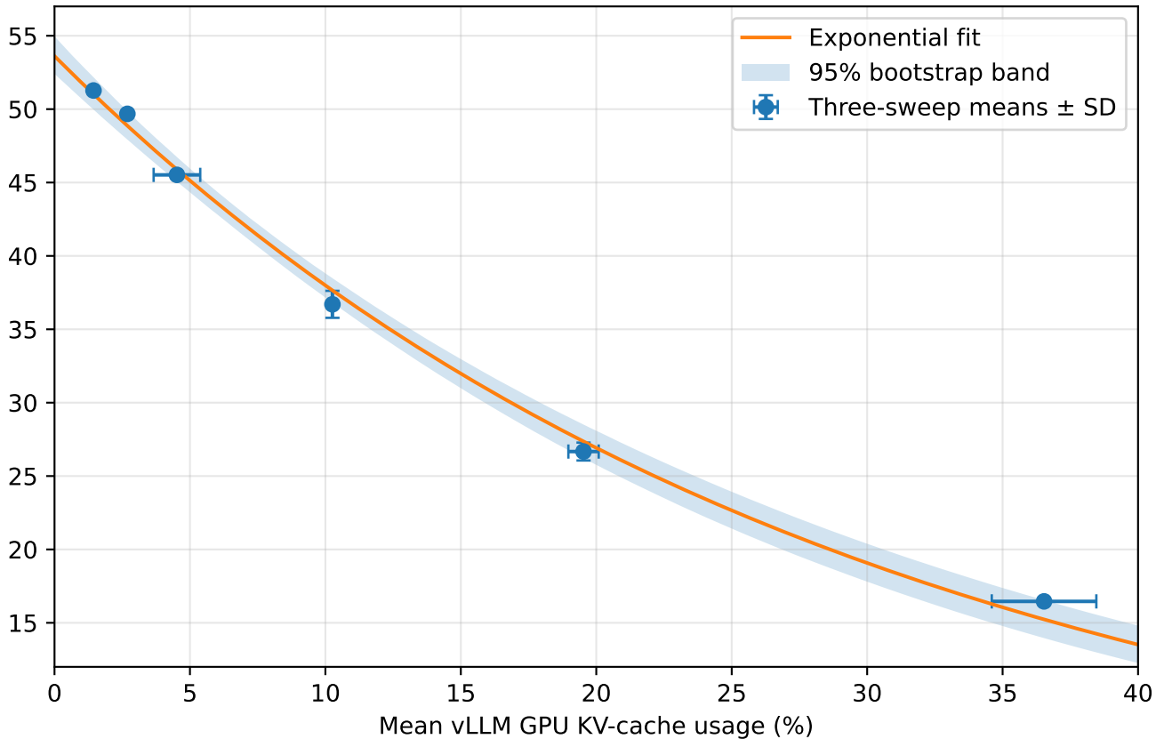
Per-stream decode rate (tokens/s)
