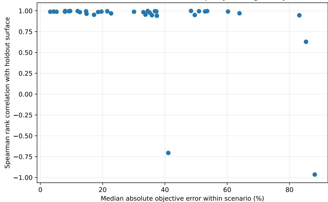
Absolute calibration error versus policy-ranking fidelity
