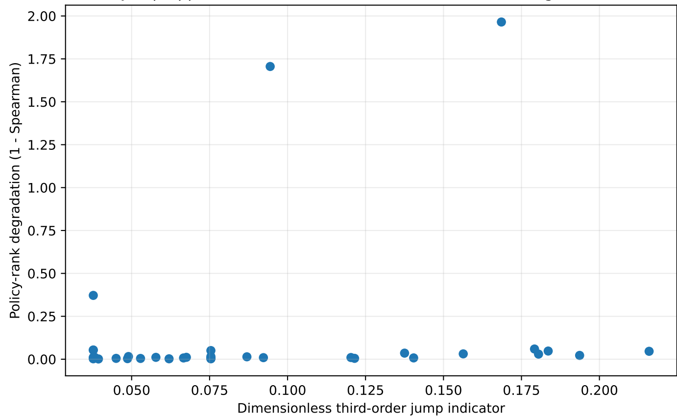
Jump-approximation remainder and observed rank degradation
