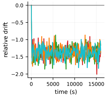
Relative total-water drift 1e-14
