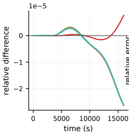
Projected relative-vorticity-squared difference from truth
