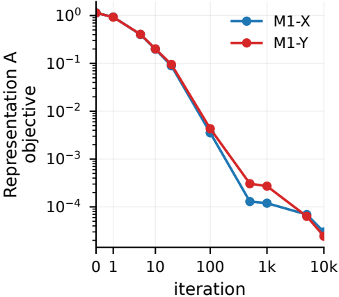
Direct physical-law objectives
