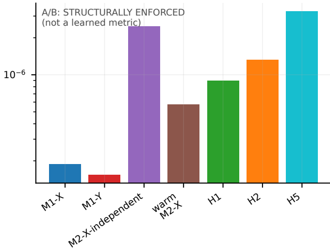
C: water-source identity defect RMS
