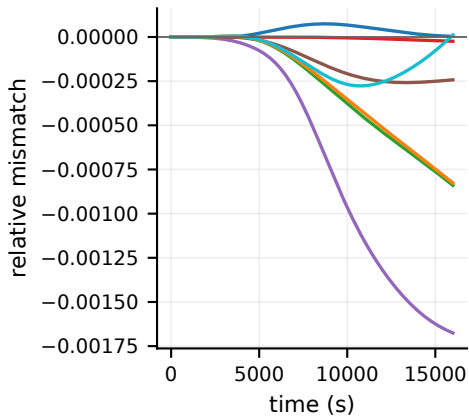
kinetic energy relative to truth
