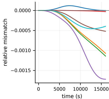
projected relative-vorticity squared
