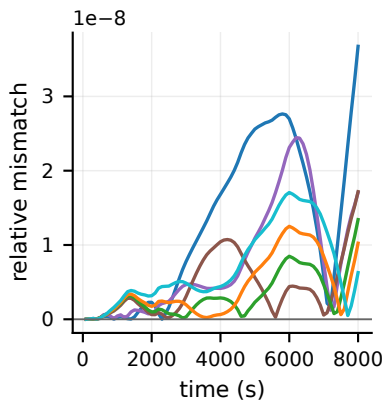
kinetic energy relative to truth
