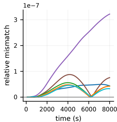
projected relative-vorticity squared
