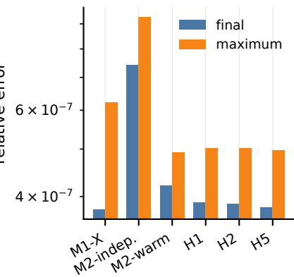
mixed-state error endpoints
