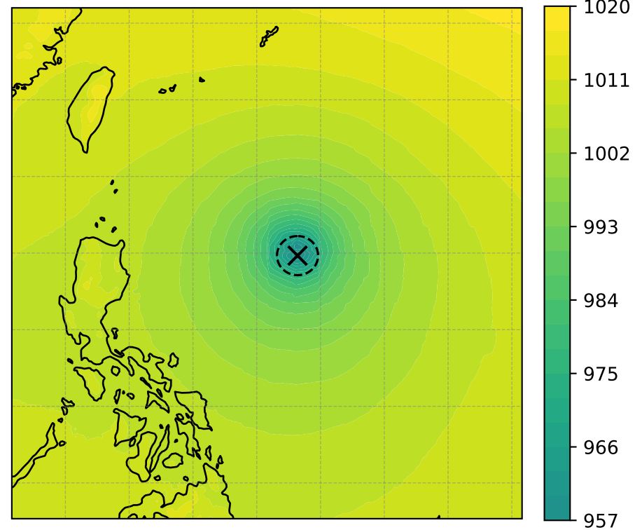
MSLP (hPa, min = 958.75)
