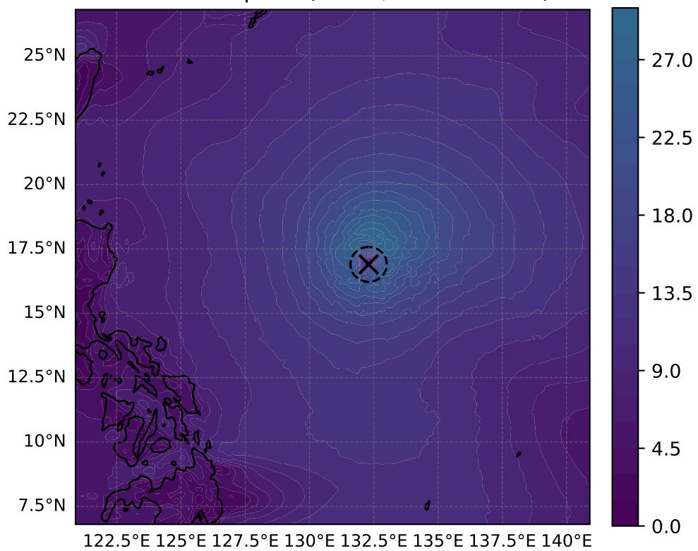
10 m windspeed ( \text{m s}^{-1} , max = 29.96)
