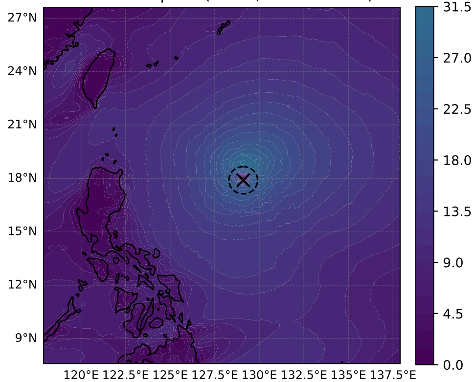
10 m windspeed ( \text{m s}^{-1} , max = 31.30)
