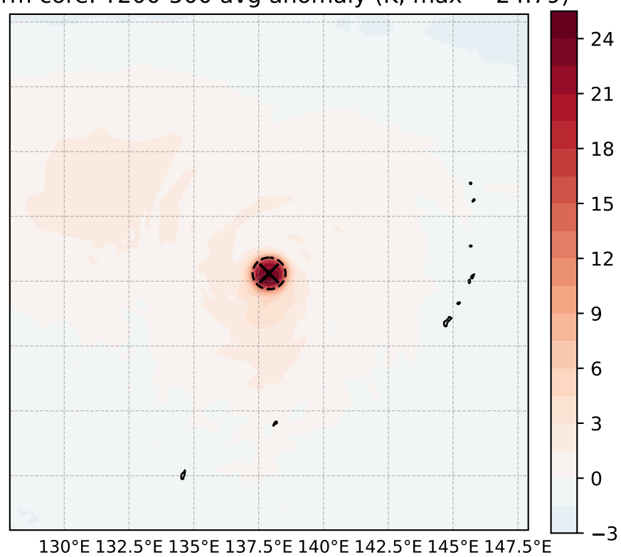
warm core: T200-500 avg anomaly (K, max = 24.79)
