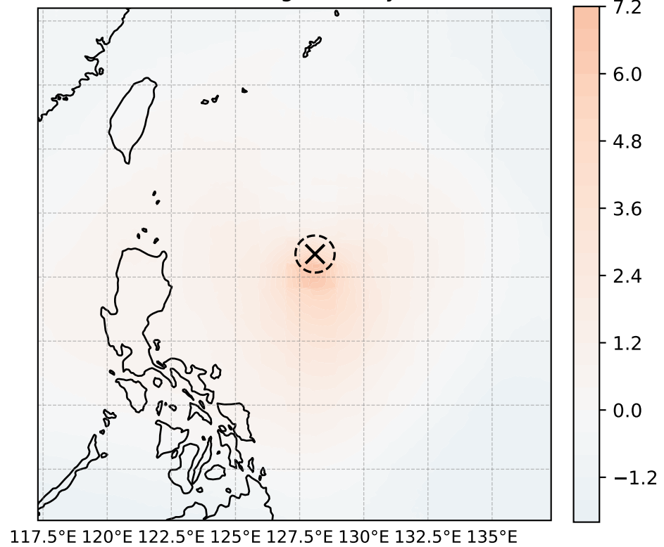
warm core: T200-500 avg anomaly (K, max = 6.91)
