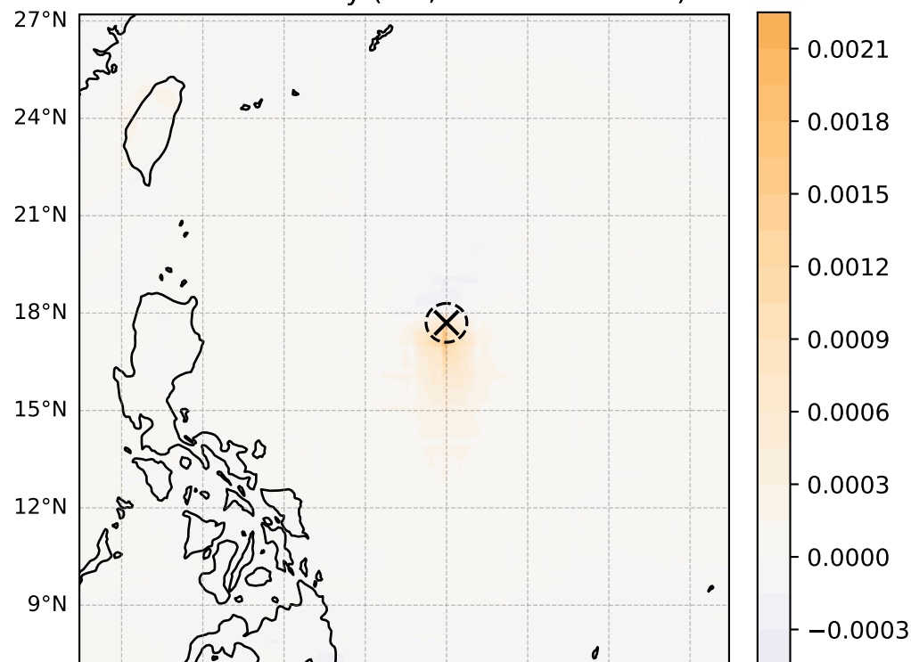
850 hPa vorticity ( \text{s}^{-1} , max = 2.20\text{e-}03 )
