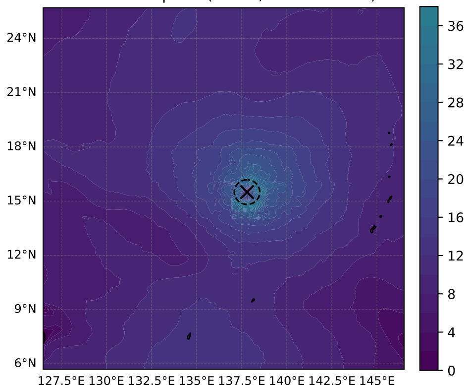
10 m windspeed ( \text{m s}^{-1} , max = 36.74)
