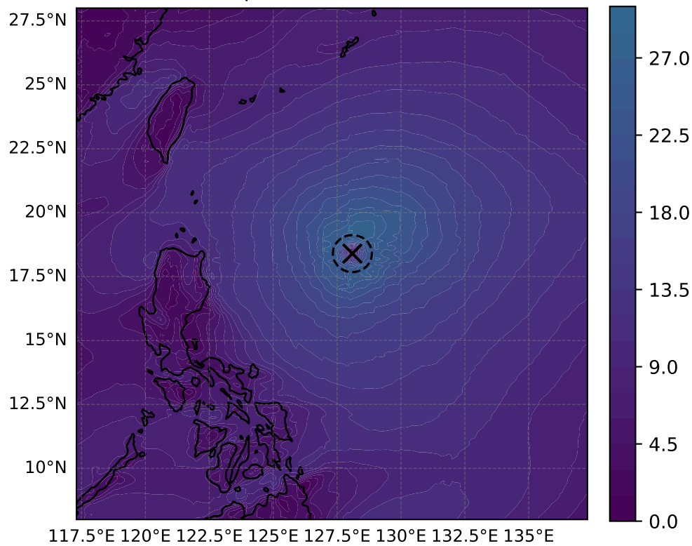
10 m windspeed ( \text{m s}^{-1} , max = 28.58)
