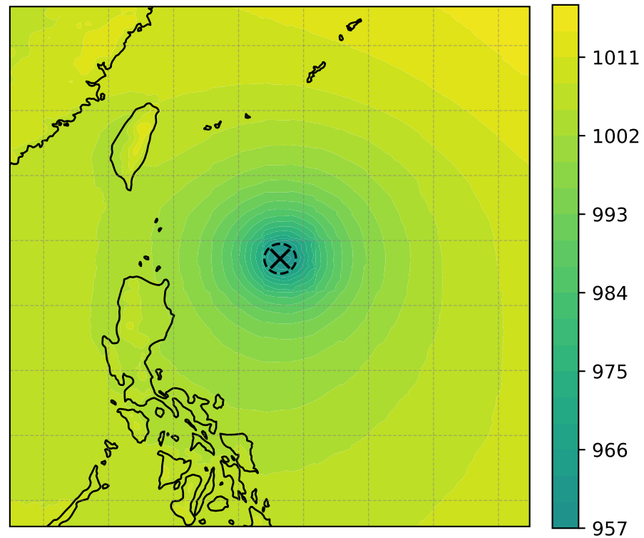
MSLP (hPa, min = 958.41)
