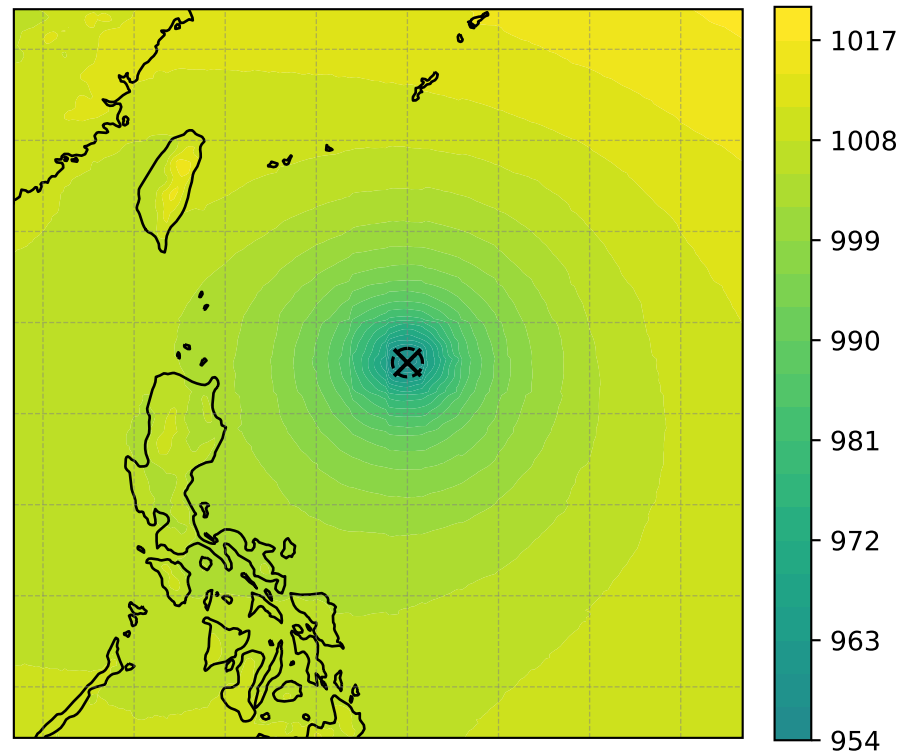
MSLP (hPa, min = 955.70)
