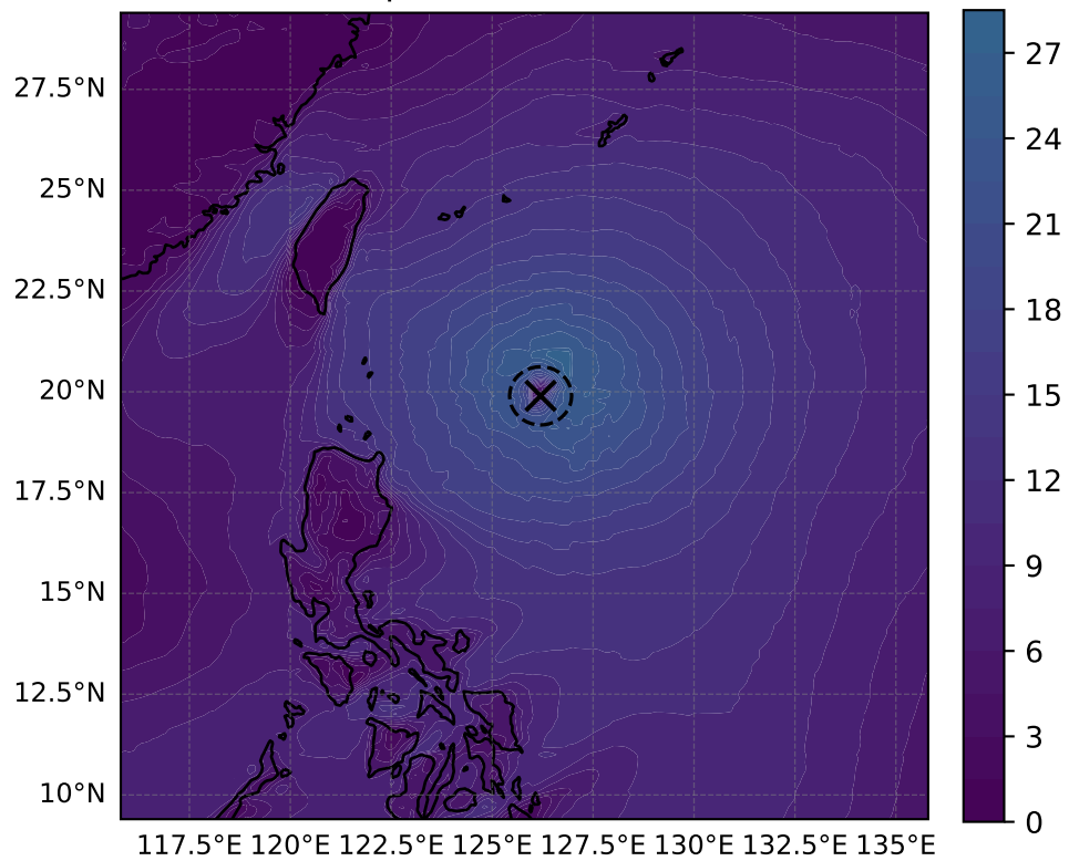
10 m windspeed ( \text{m s}^{-1} , max = 28.25)
