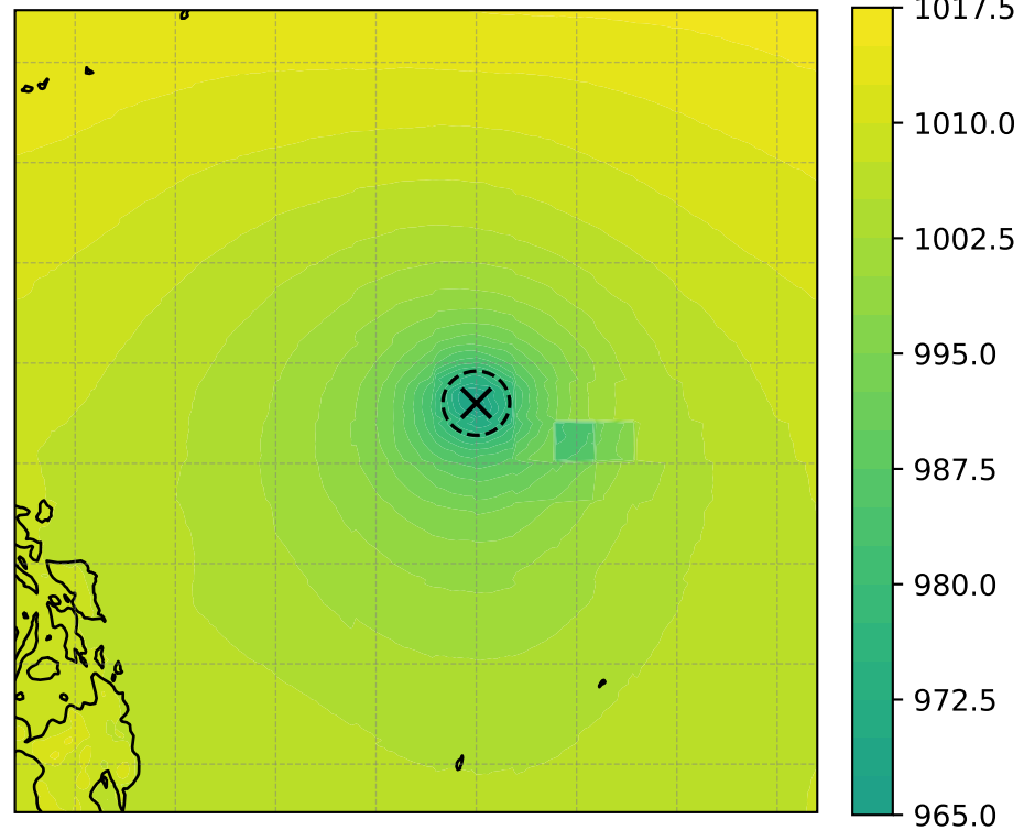
MSLP (hPa, min = 966.50)
