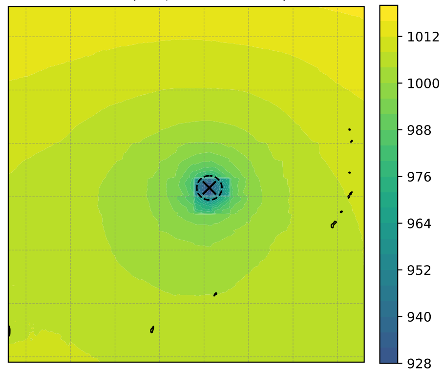
MSLP (hPa, min = 931.78)
