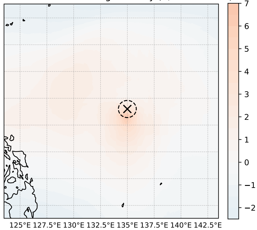
warm core: T200-500 avg anomaly (K, max = 6.66)
