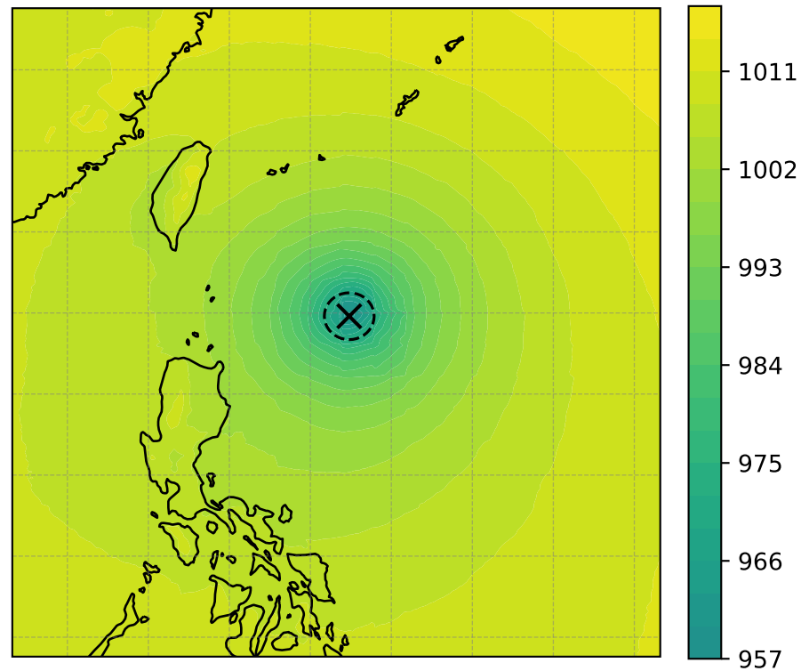
MSLP (hPa, min = 959.56)
