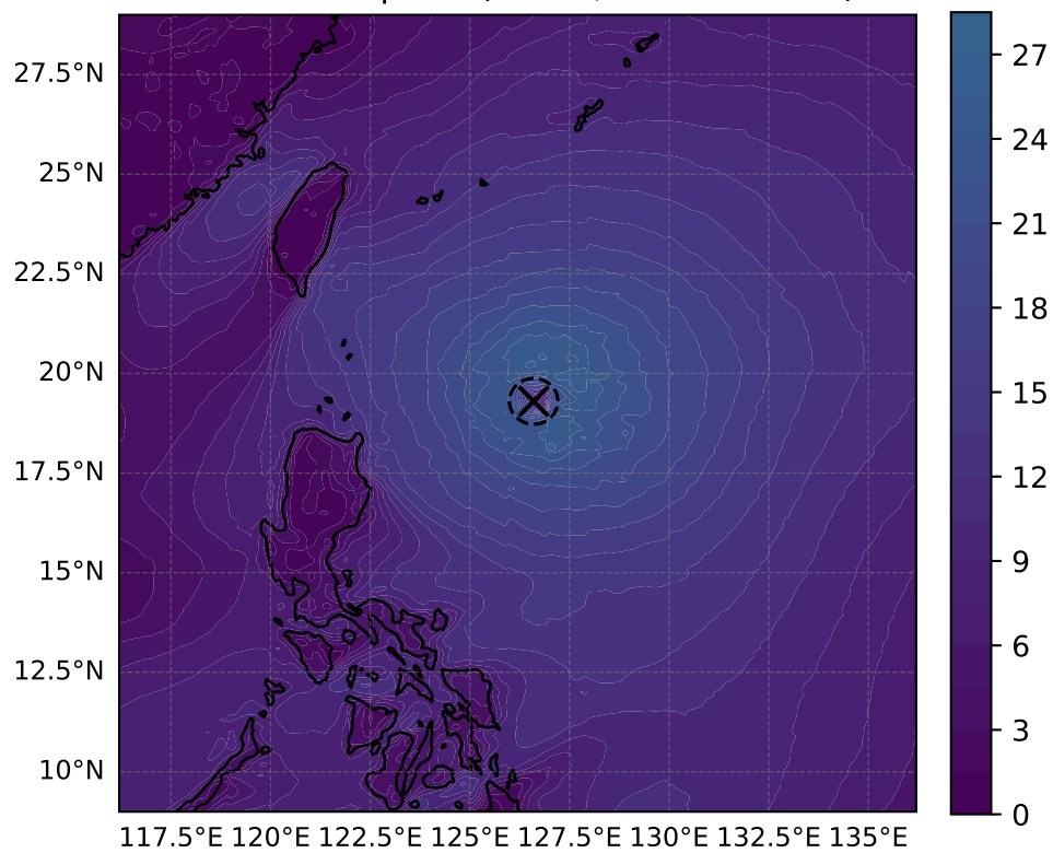
10 m windspeed ( \text{m s}^{-1} , max = 27.00)
