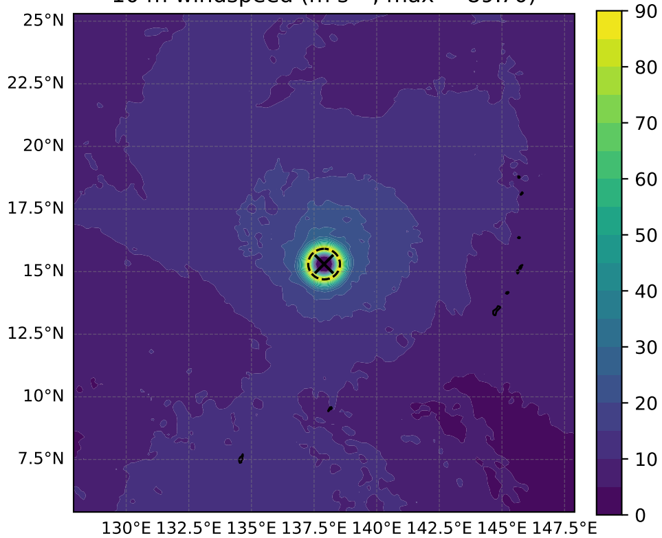
10 m windspeed ( \text{m s}^{-1} , max = 89.70)
