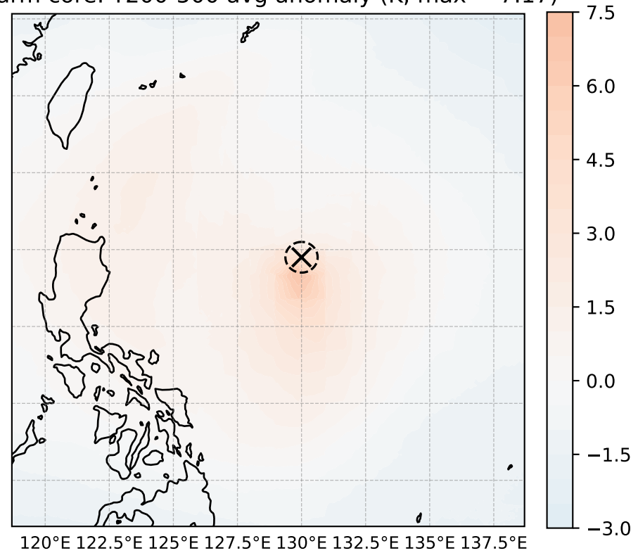
warm core: T200-500 avg anomaly (K, max = 7.17)
