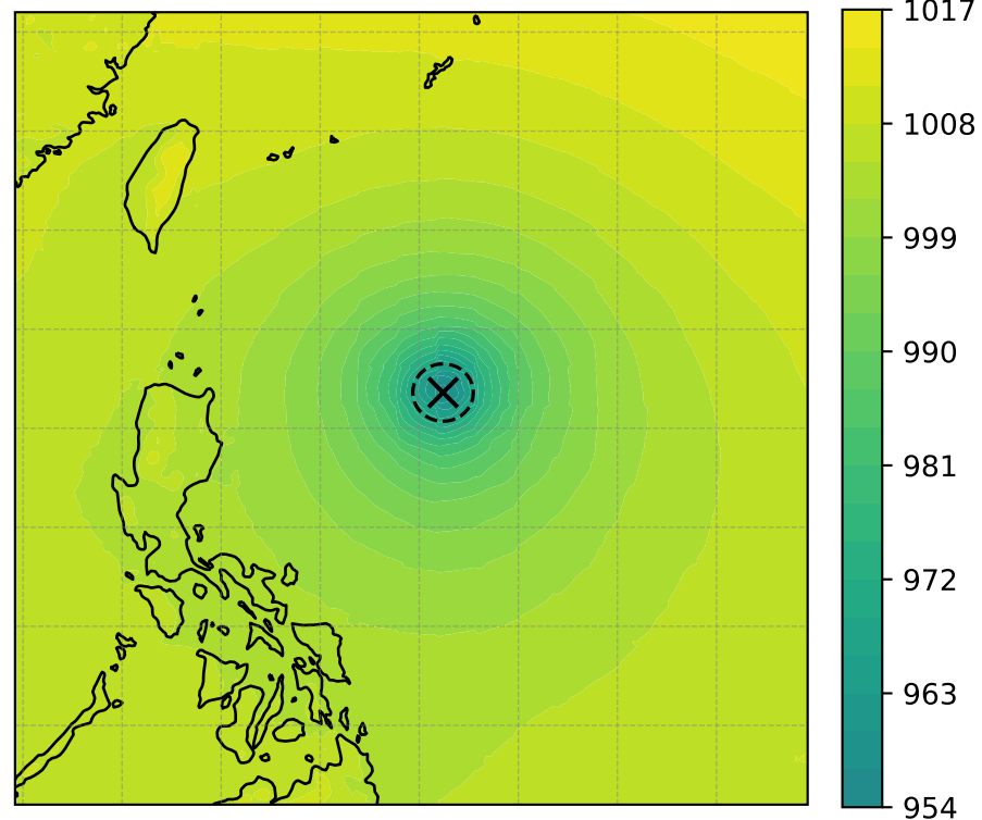
MSLP (hPa, min = 955.98)
