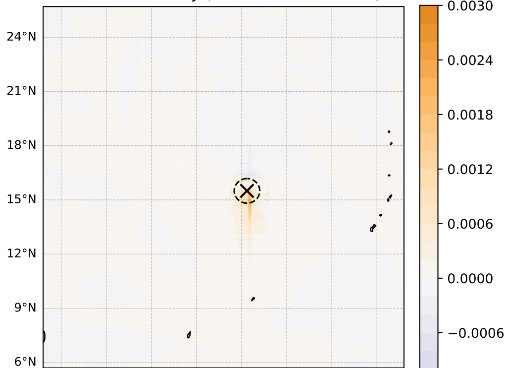
850 hPa vorticity ( \text{s}^{-1} , max = 2.81\text{e-}03 )
