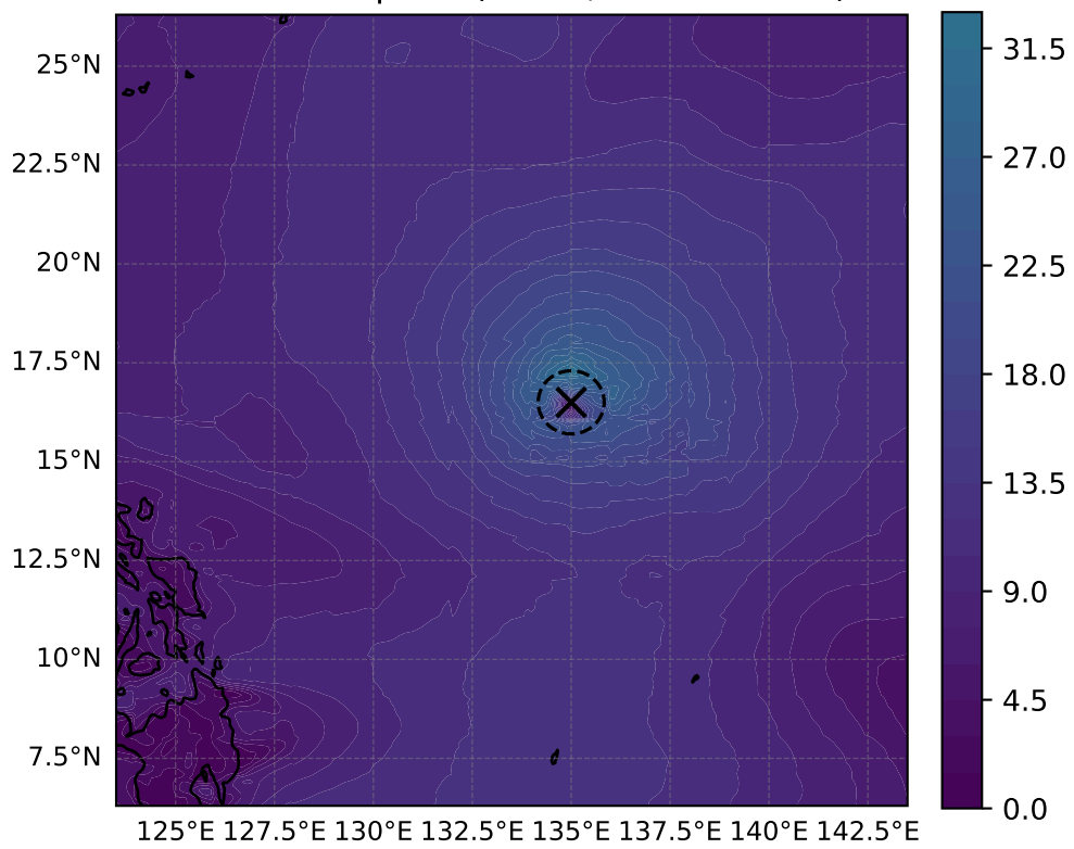
10 m windspeed ( \text{m s}^{-1} , max = 32.91)
