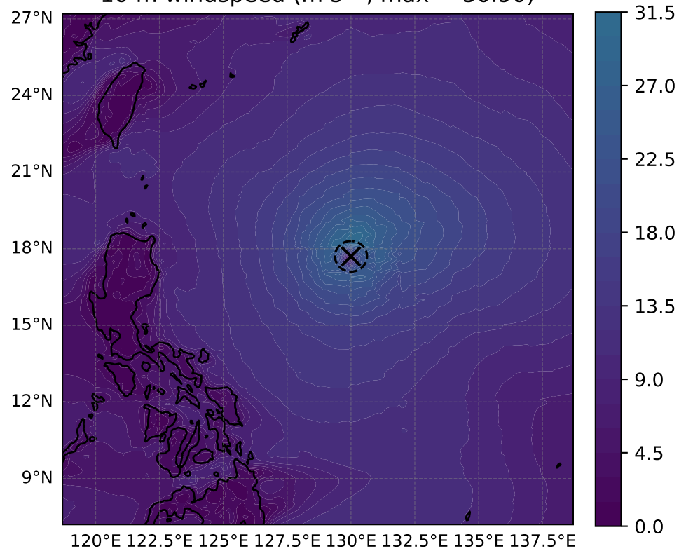
10 m windspeed ( \text{m s}^{-1} , max = 30.90)
