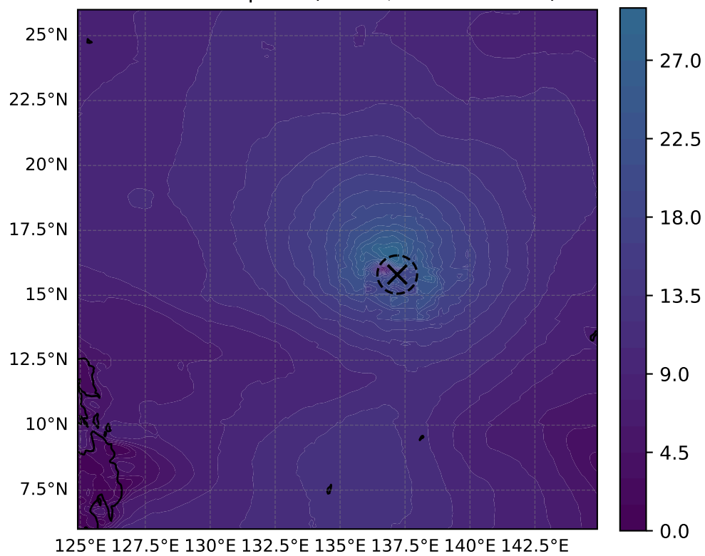
10 m windspeed ( \text{m s}^{-1} , max = 29.97)
