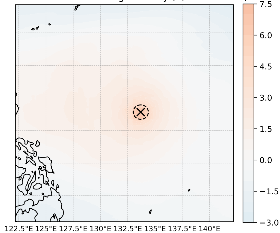
warm core: T200-500 avg anomaly (K, max = 7.14)
