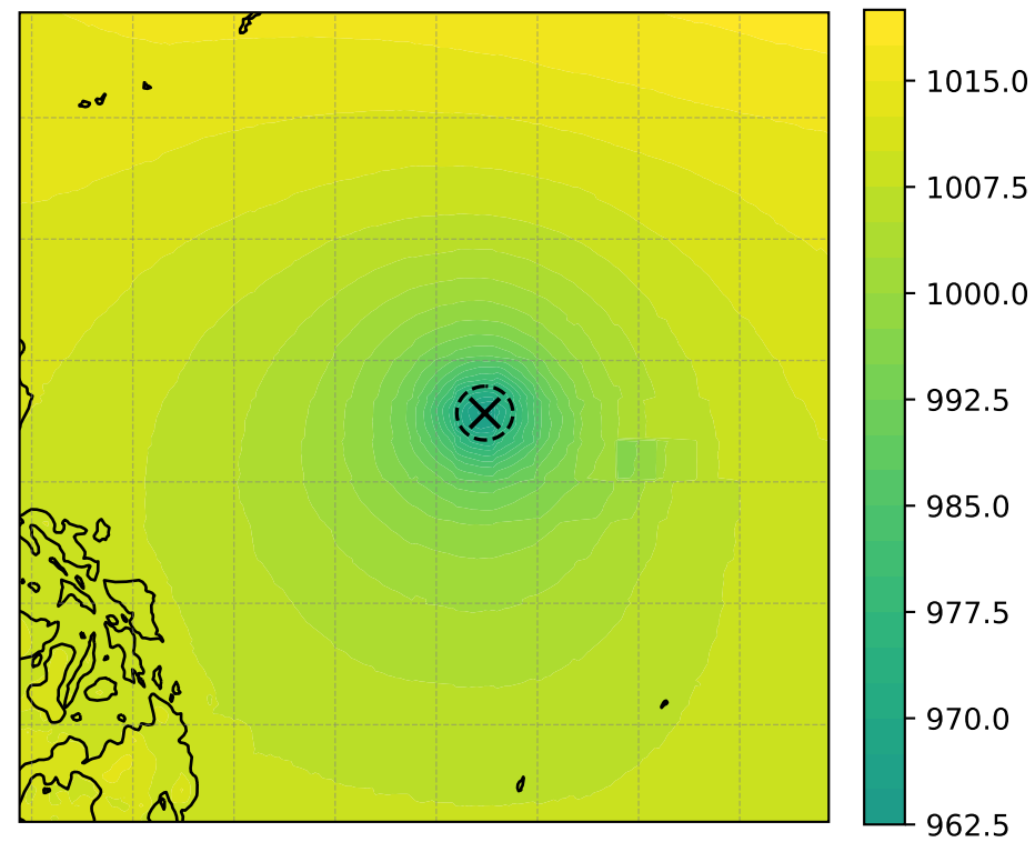
MSLP (hPa, min = 964.13)
