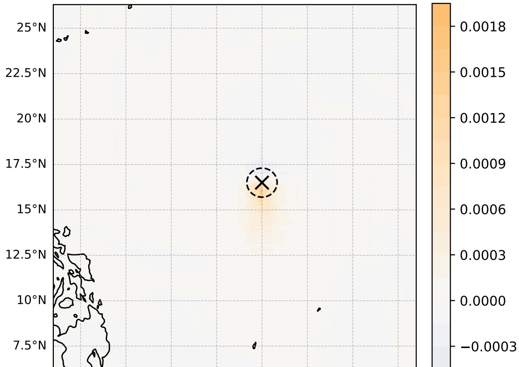
850 hPa vorticity ( \text{s}^{-1} , max = 1.89\text{e-}03 )
