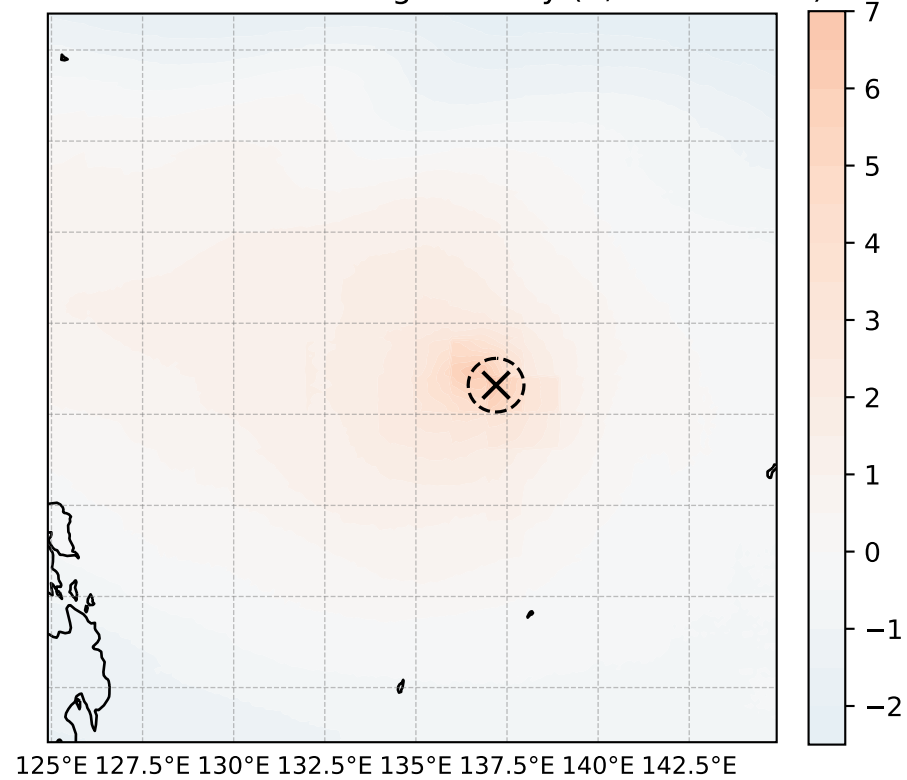
warm core: T200-500 avg anomaly (K, max = 6.79)
