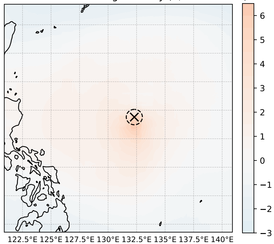
warm core: T200-500 avg anomaly (K, max = 6.32)
