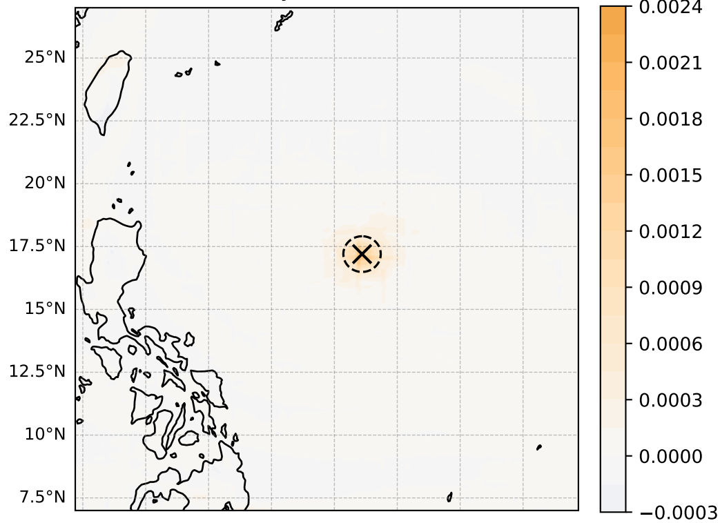
850 hPa vorticity ( \text{s}^{-1} , max = 2.37\text{e-}03 )
