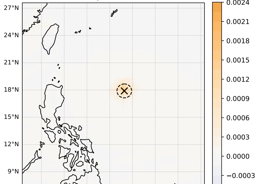
850 hPa vorticity ( \text{s}^{-1} , max = 2.31\text{e-}03 )
