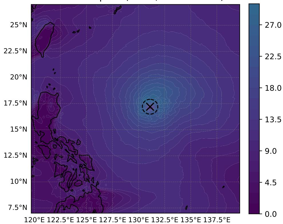
10 m windspeed ( \text{m s}^{-1} , max = 29.53)
