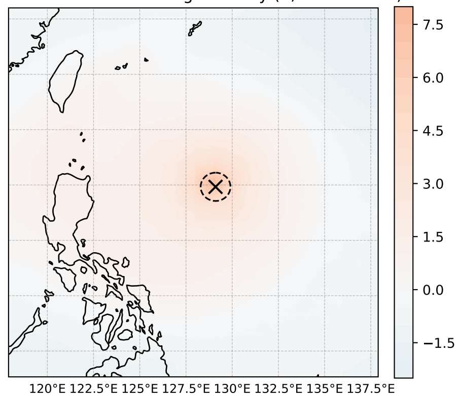
warm core: T200-500 avg anomaly (K, max = 7.54)
