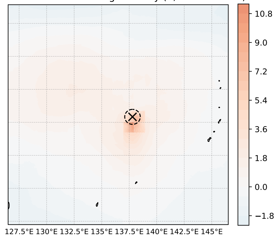
warm core: T200-500 avg anomaly (K, max = 10.80)
