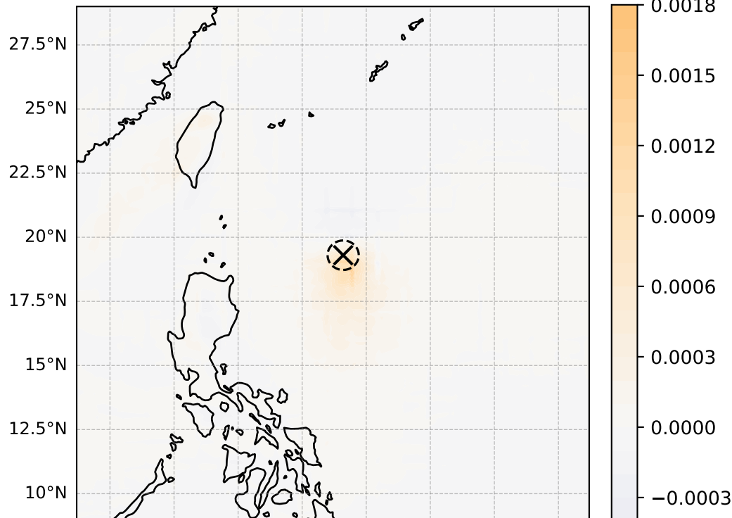
850 hPa vorticity ( \text{s}^{-1} , max = 1.76\text{e-}03 )
