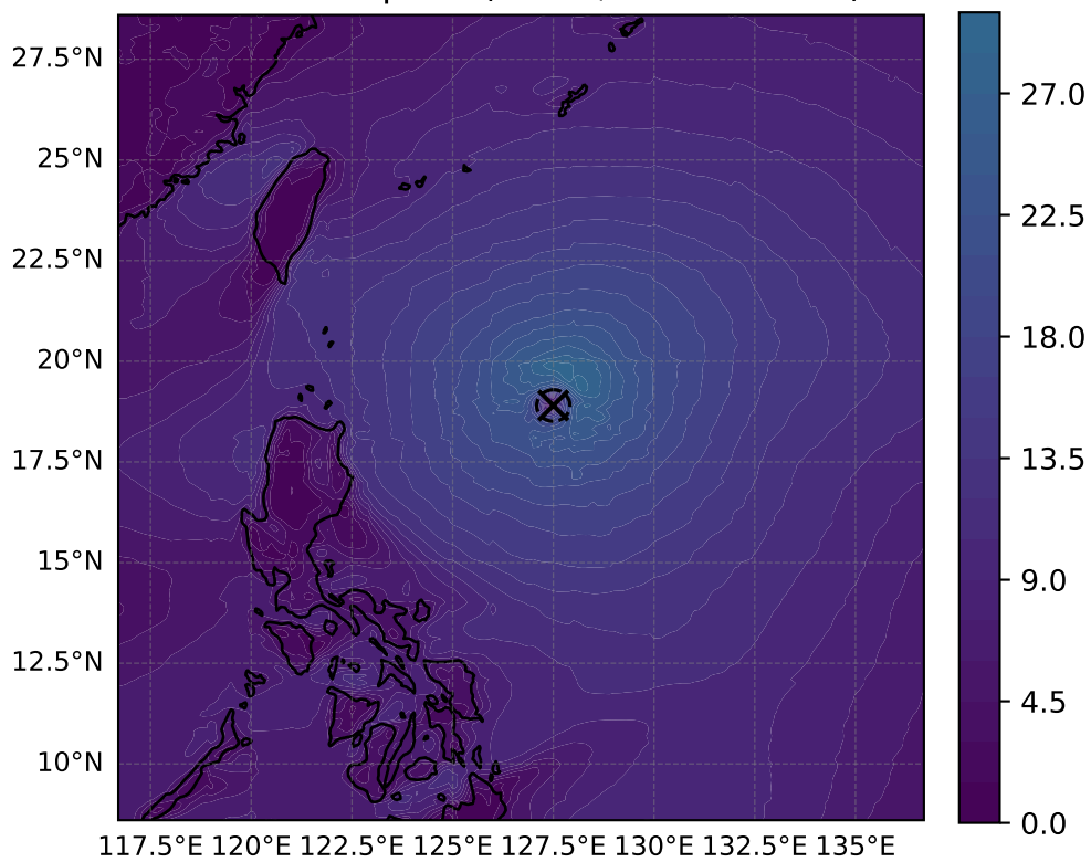
10 m windspeed ( \text{m s}^{-1} , max = 29.52)
