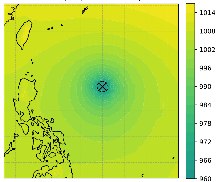
MSLP (hPa, min = 960.25)
