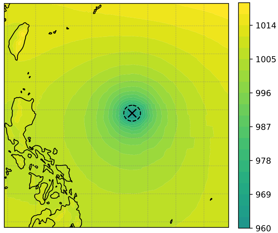
MSLP (hPa, min = 961.90)
