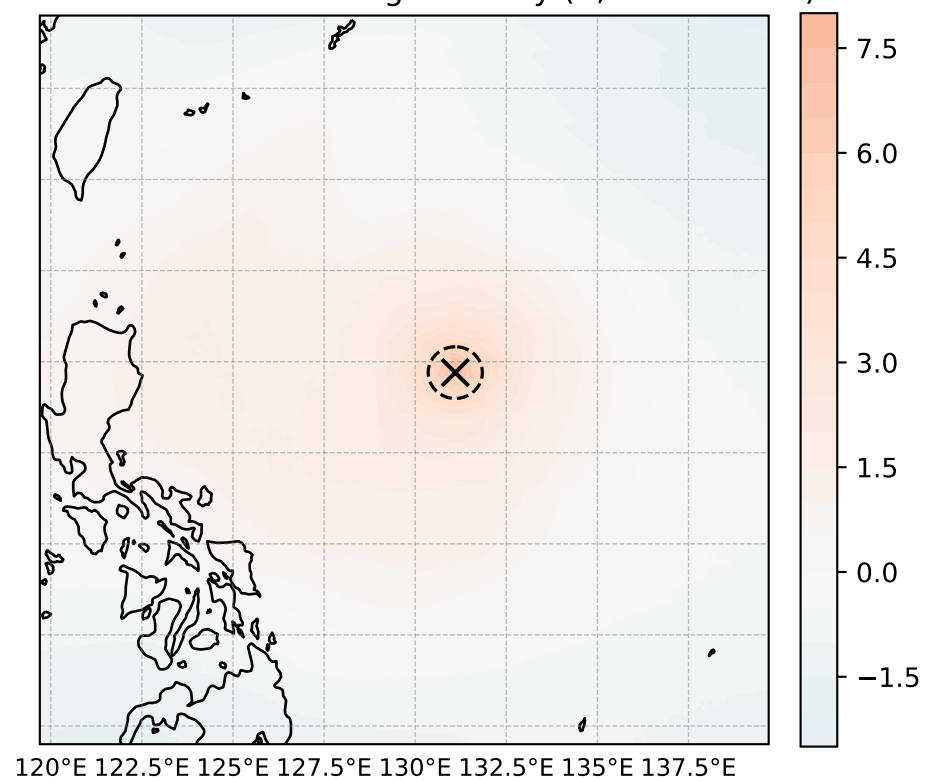
warm core: T200-500 avg anomaly (K, max = 7.88)
