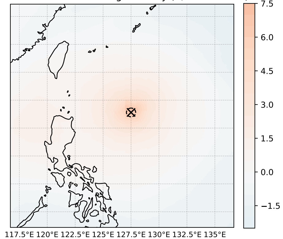
warm core: T200-500 avg anomaly (K, max = 7.05)
