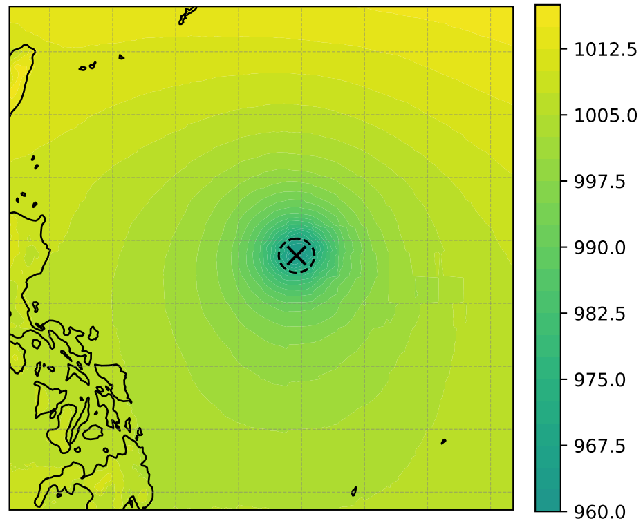
MSLP (hPa, min = 962.00)
