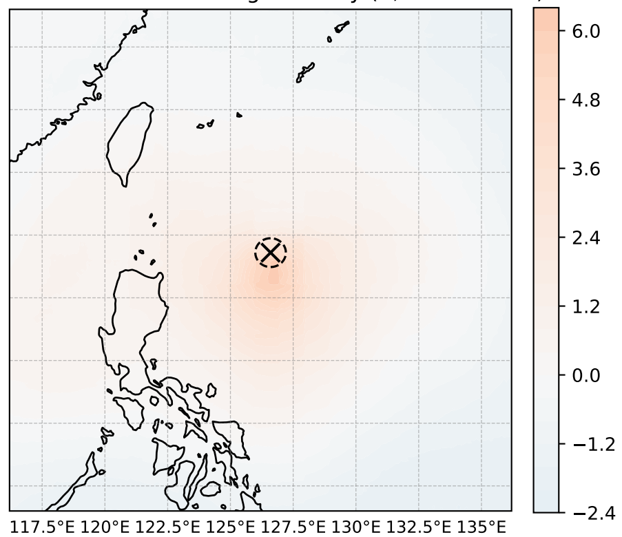
warm core: T200-500 avg anomaly (K, max = 6.29)
