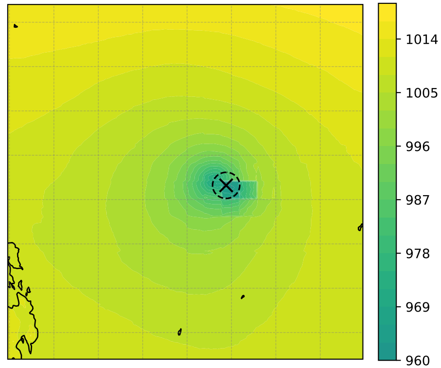
MSLP (hPa, min = 962.80)
