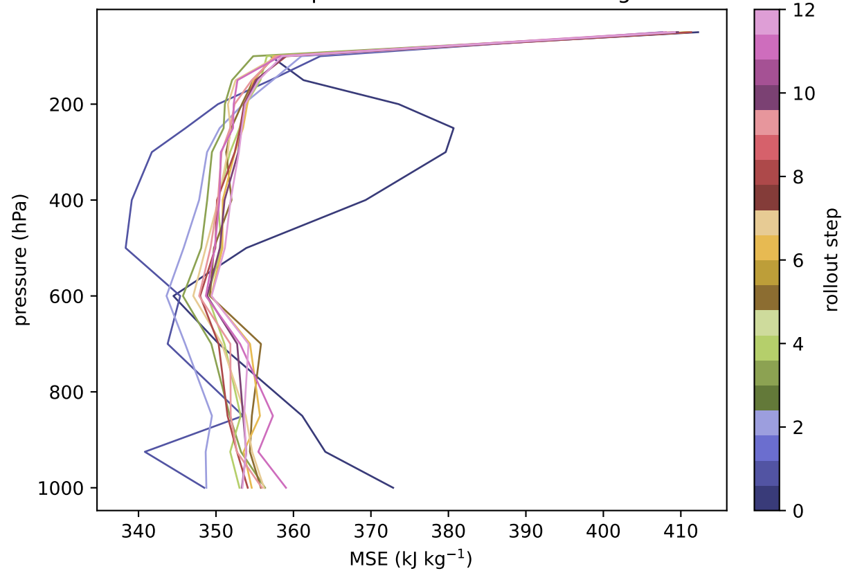
MSE vertical profile at storm centre -- bogus
