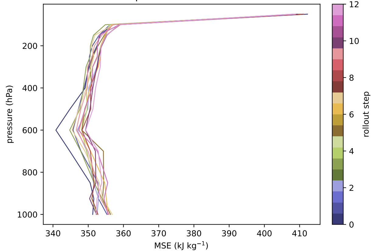
MSE vertical profile at storm centre -- control
