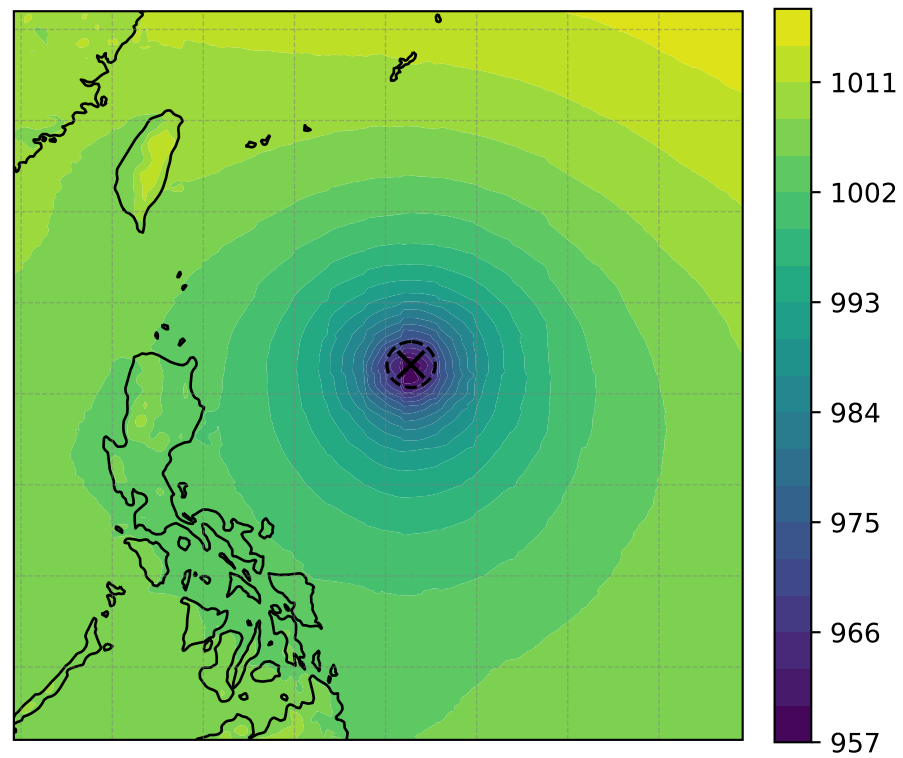
MSLP (hPa, min = 957.61)
