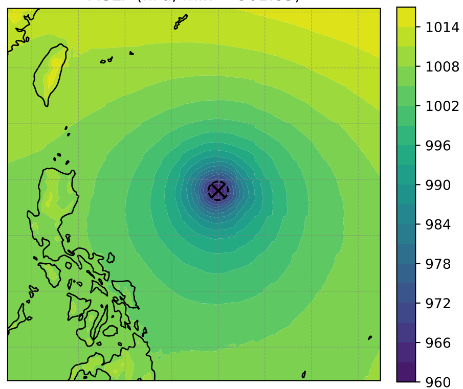
MSLP (hPa, min = 961.85)
