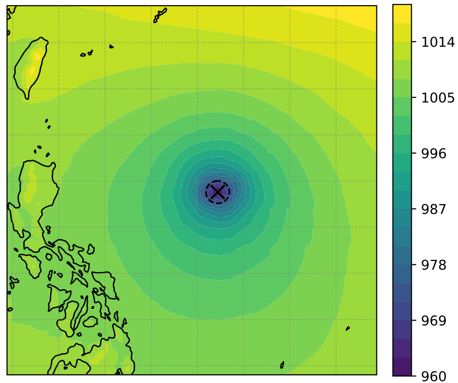
MSLP (hPa, min = 963.09)
