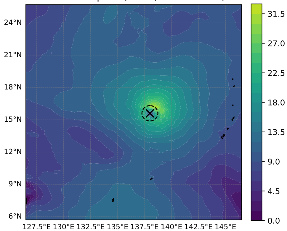
10 m windspeed ( \text{m s}^{-1} , max = 31.70)
