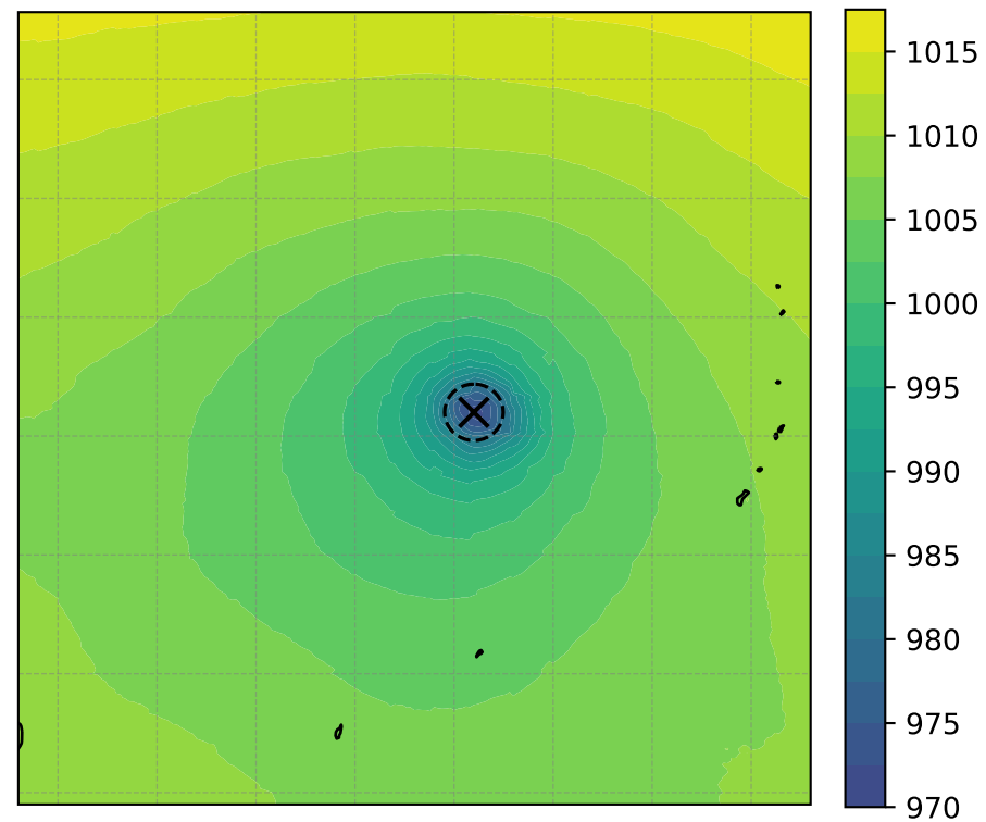
MSLP (hPa, min = 971.64)
