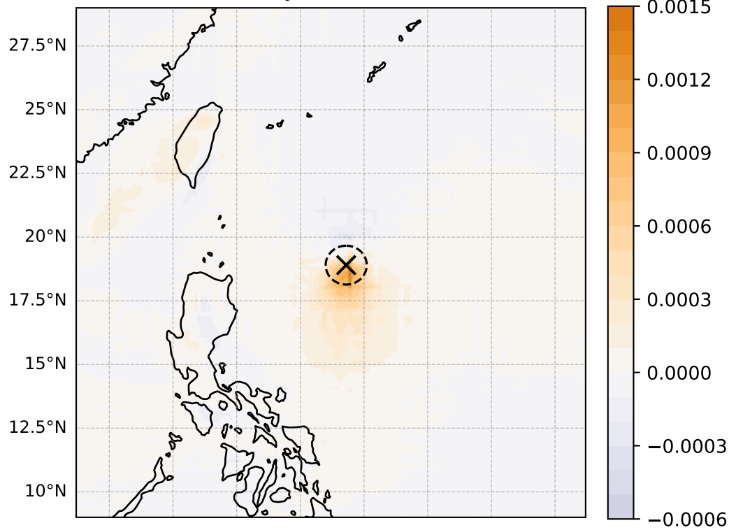
850 hPa vorticity ( \text{s}^{-1} , max = 1.44\text{e-}03 )
