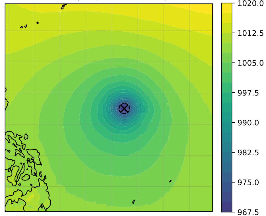
MSLP (hPa, min = 968.06)
