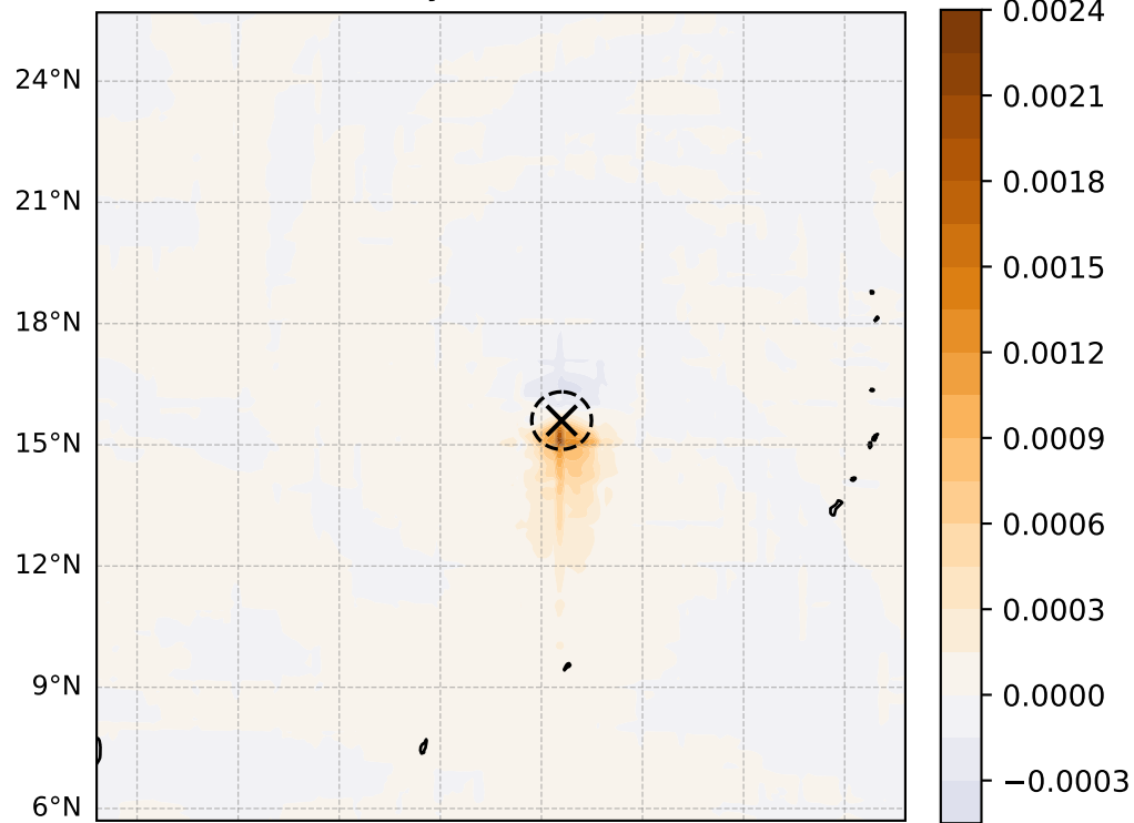
850 hPa vorticity ( \text{s}^{-1} , max = 2.30\text{e-}03 )
