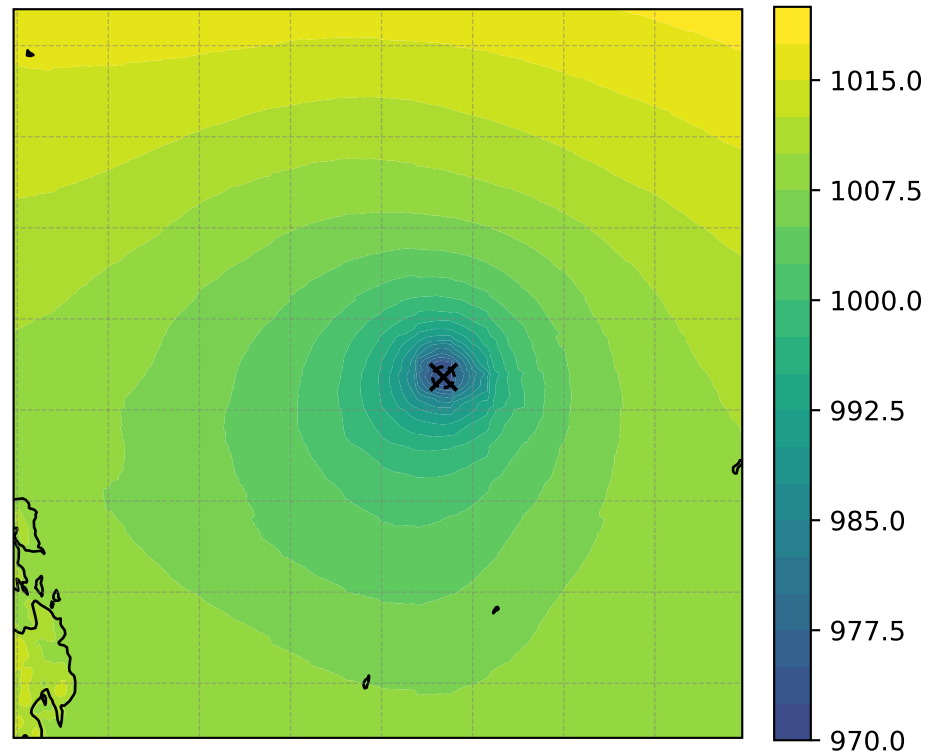
MSLP (hPa, min = 971.25)
