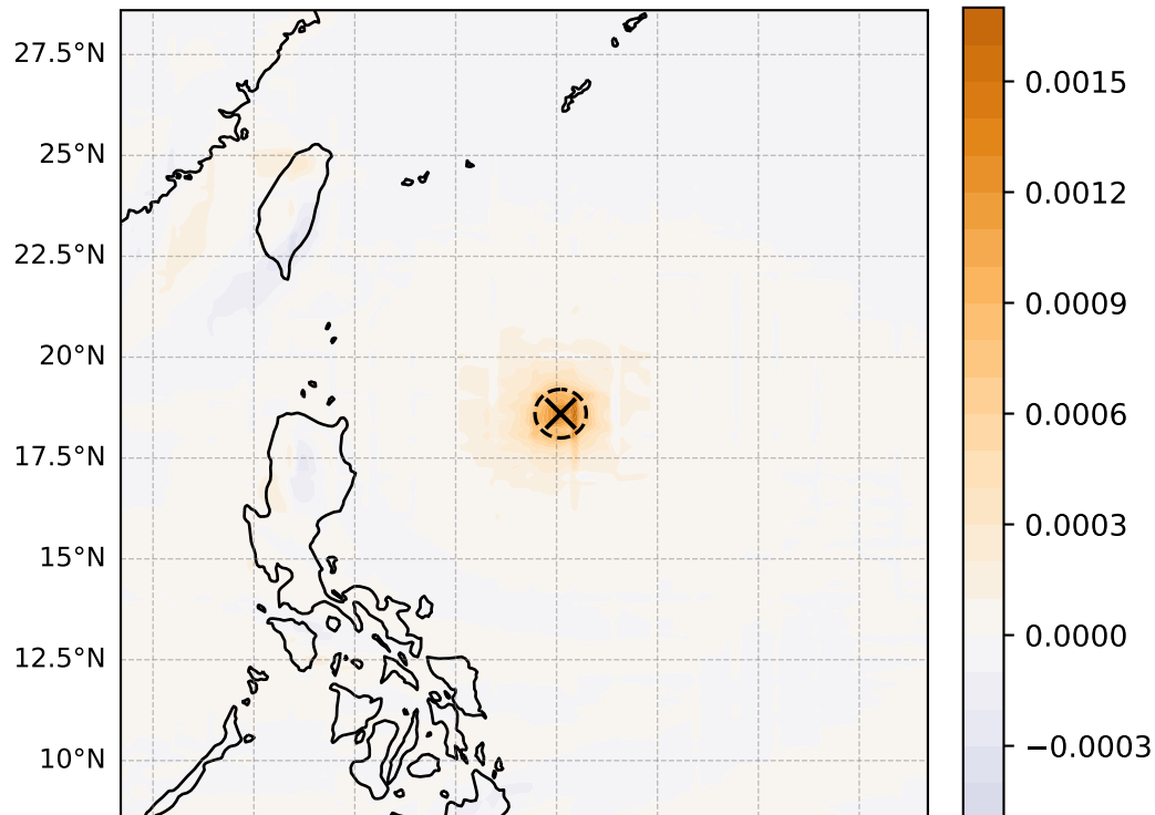
850 hPa vorticity ( \text{s}^{-1} , max = 1.62\text{e-}03 )
