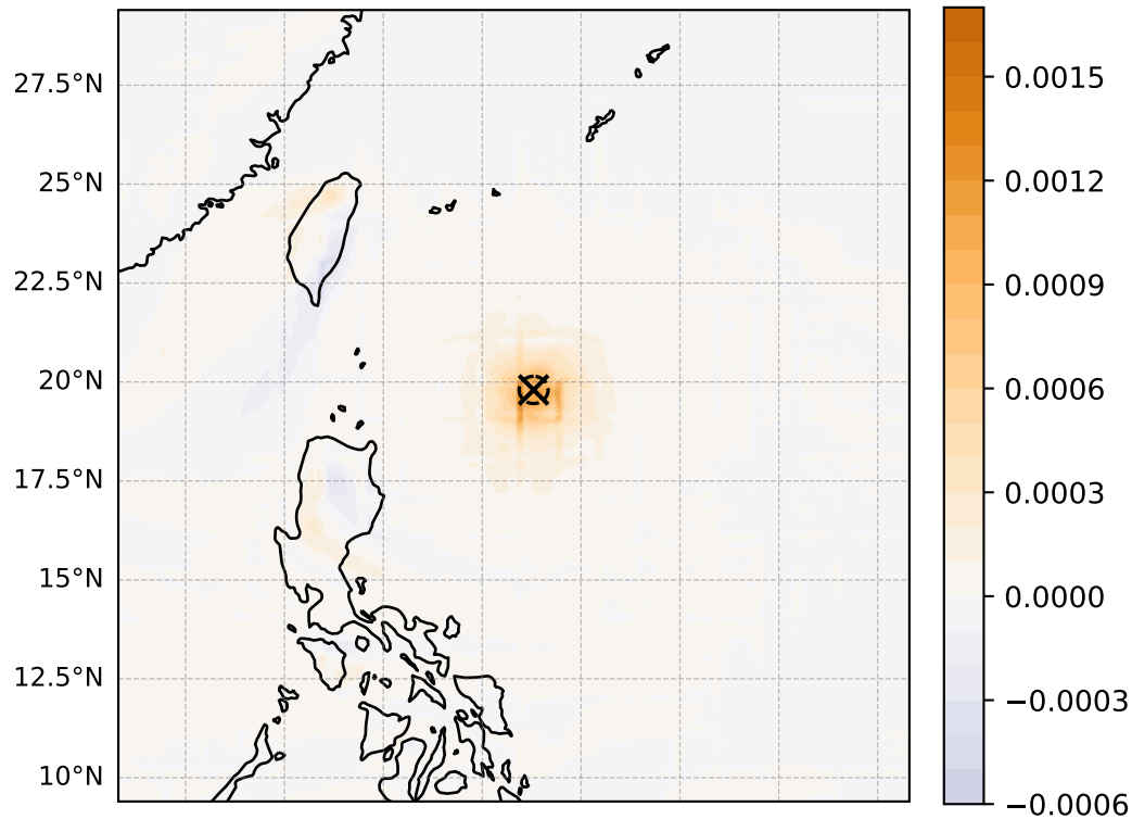
850 hPa vorticity ( \text{s}^{-1} , max = 1.62\text{e-}03 )
