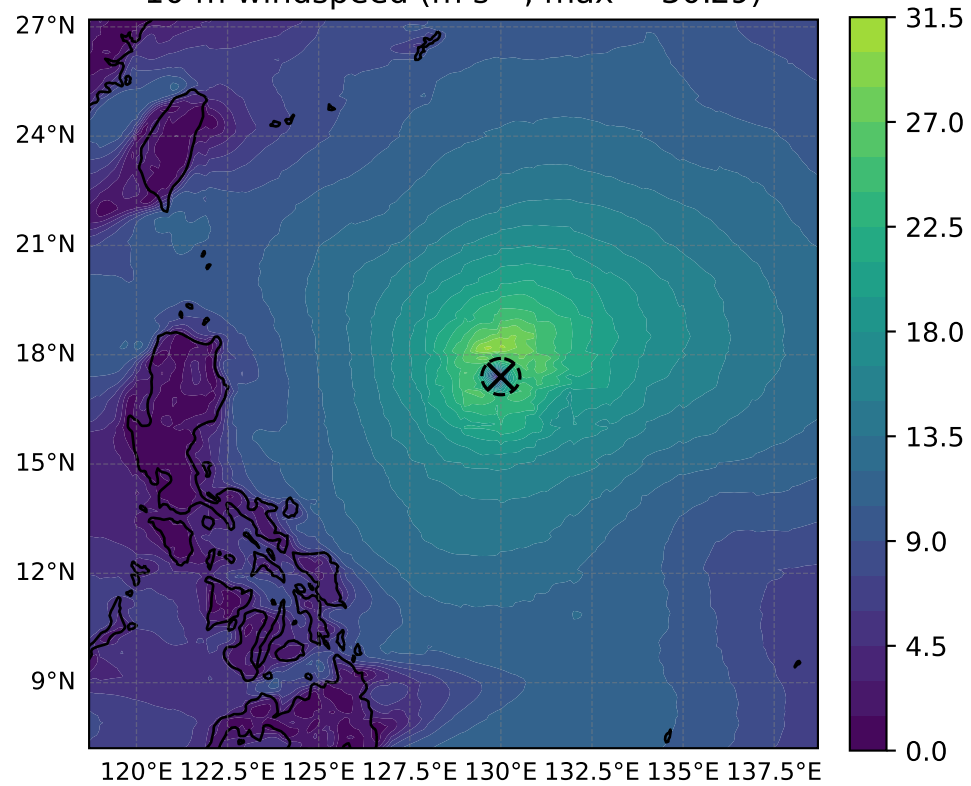
10 m windspeed ( \text{m s}^{-1} , max = 30.29)
