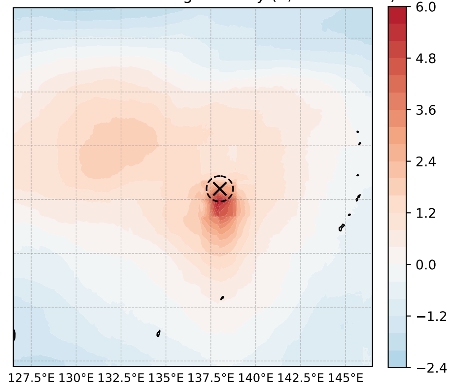
warm core: T200-500 avg anomaly (K, max = 5.92)
