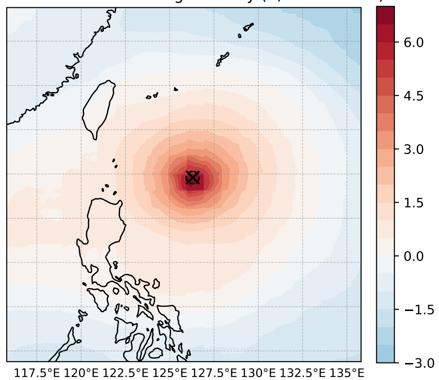
warm core: T200-500 avg anomaly (K, max = 6.89)
