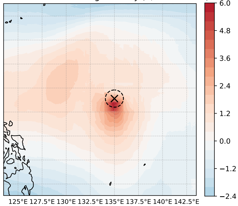
warm core: T200-500 avg anomaly (K, max = 5.86)
