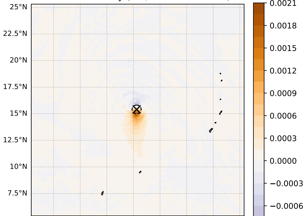
850 hPa vorticity ( \text{s}^{-1} , max = 2.03\text{e-}03 )
