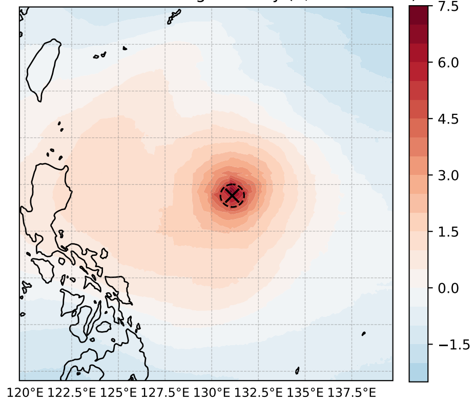
warm core: T200-500 avg anomaly (K, max = 7.41)
