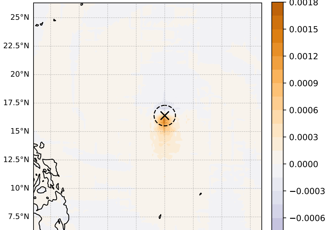
850 hPa vorticity ( \text{s}^{-1} , max = 1.73\text{e-}03 )
