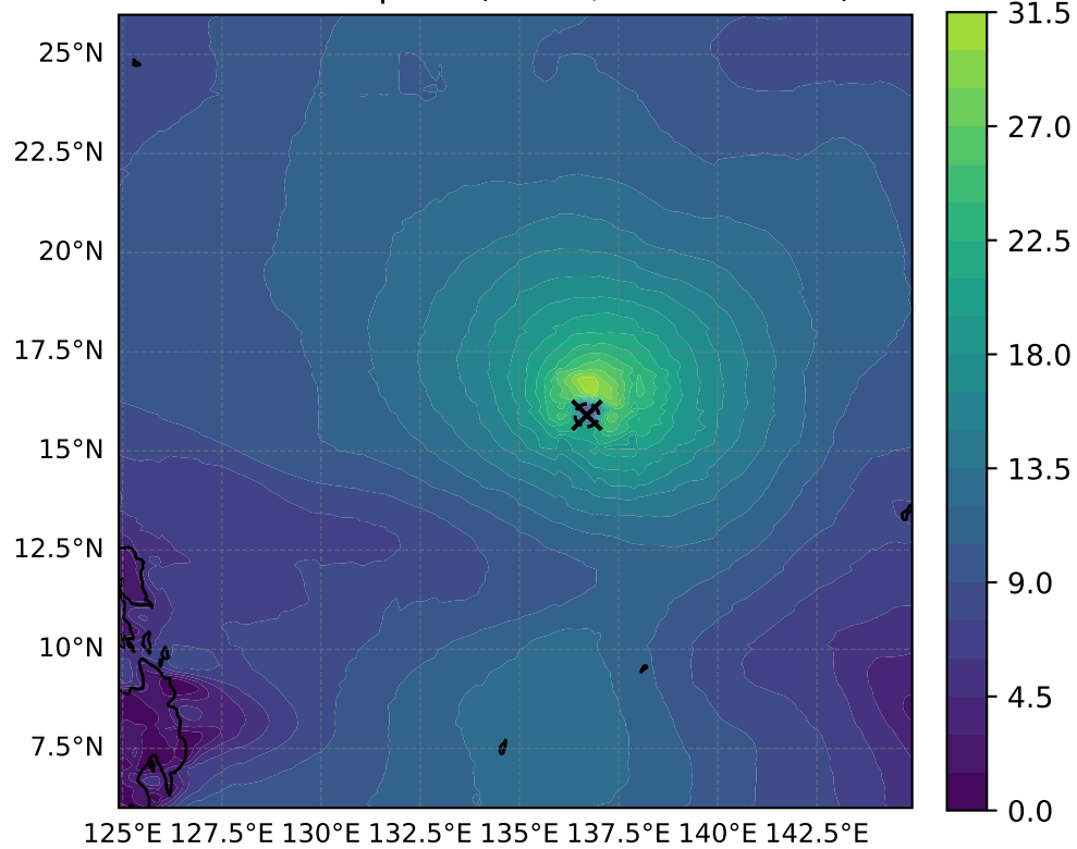
10 m windspeed ( \text{m s}^{-1} , max = 31.46)
