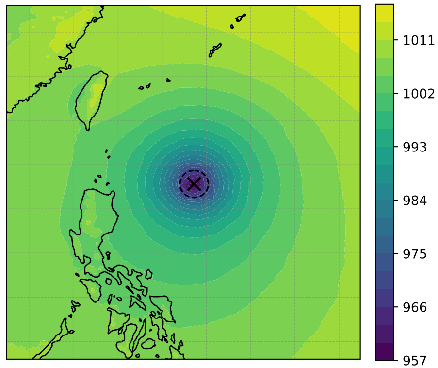
MSLP (hPa, min = 958.33)
