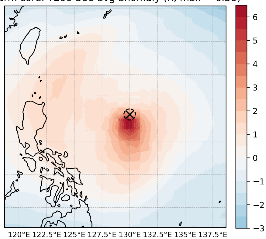
warm core: T200-500 avg anomaly (K, max = 6.50)
