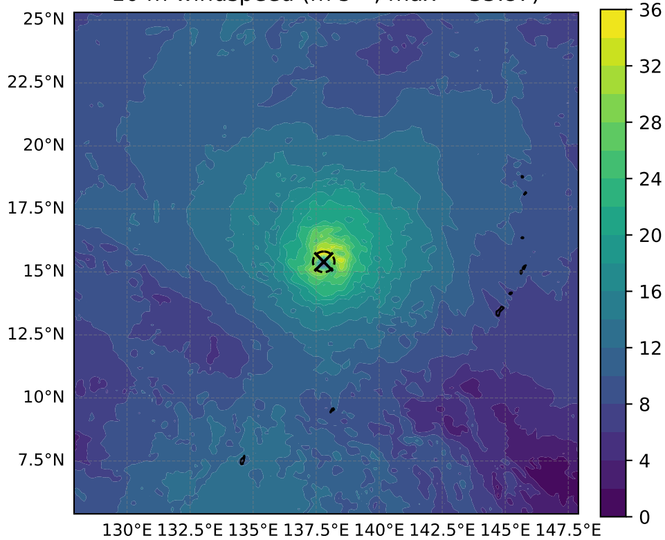
10 m windspeed ( \text{m s}^{-1} , max = 35.87)
