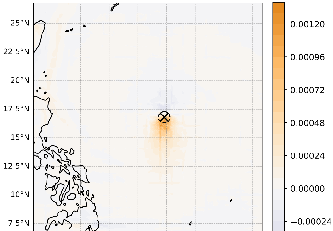
850 hPa vorticity ( \text{s}^{-1} , max = 1.34\text{e-}03 )
