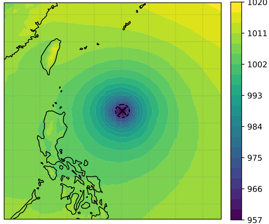
MSLP (hPa, min = 958.46)
