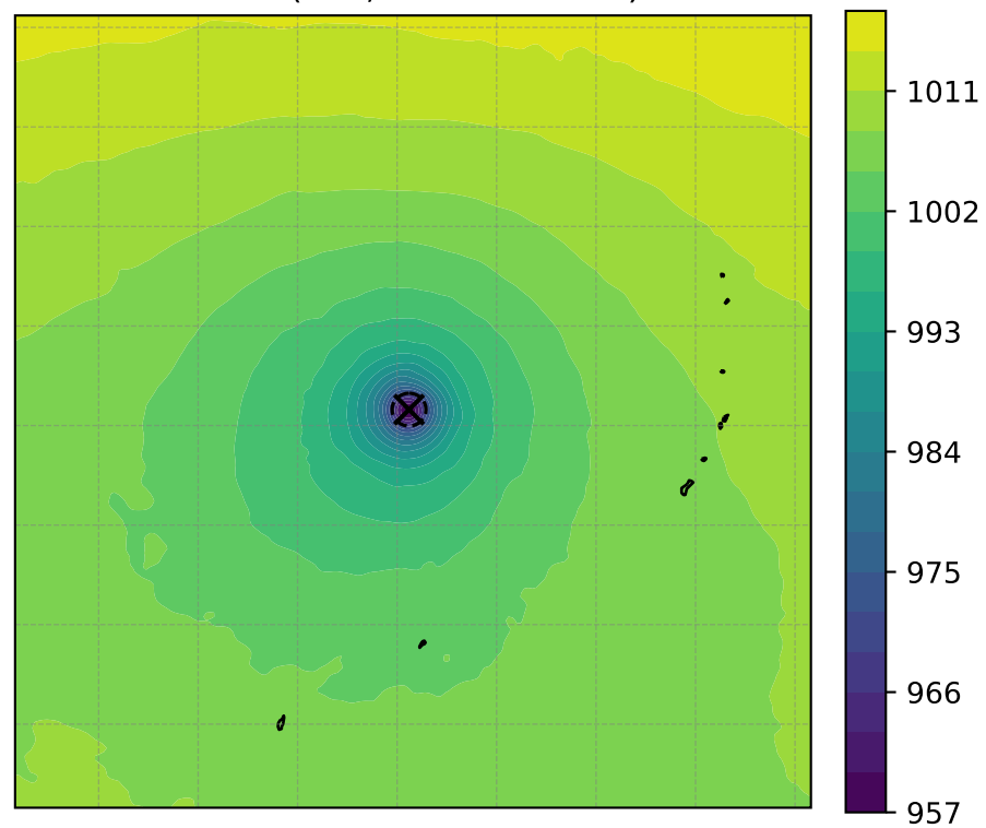
MSLP (hPa, min = 957.41)
