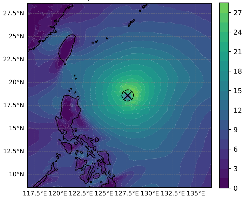
10 m windspeed ( \text{m s}^{-1} , max = 28.35)
