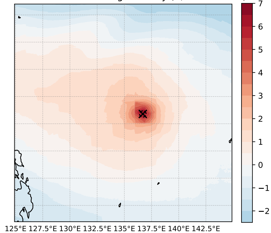
warm core: T200-500 avg anomaly (K, max = 6.55)
