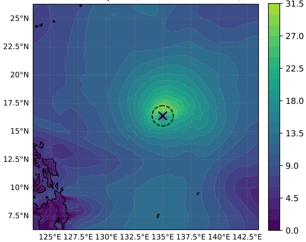
10 m windspeed ( \text{m s}^{-1} , max = 30.01)
