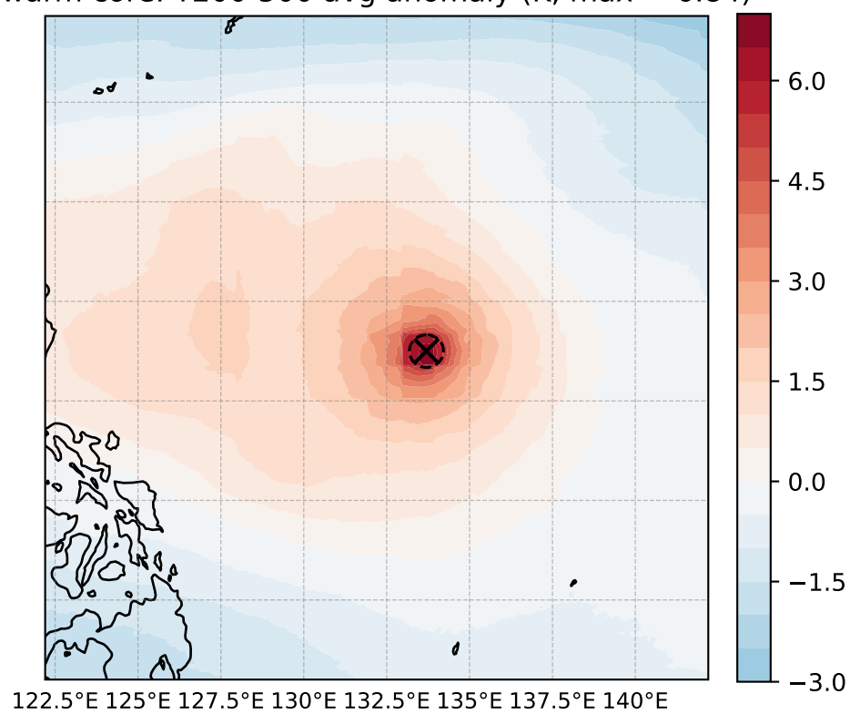
warm core: T200-500 avg anomaly (K, max = 6.84)
