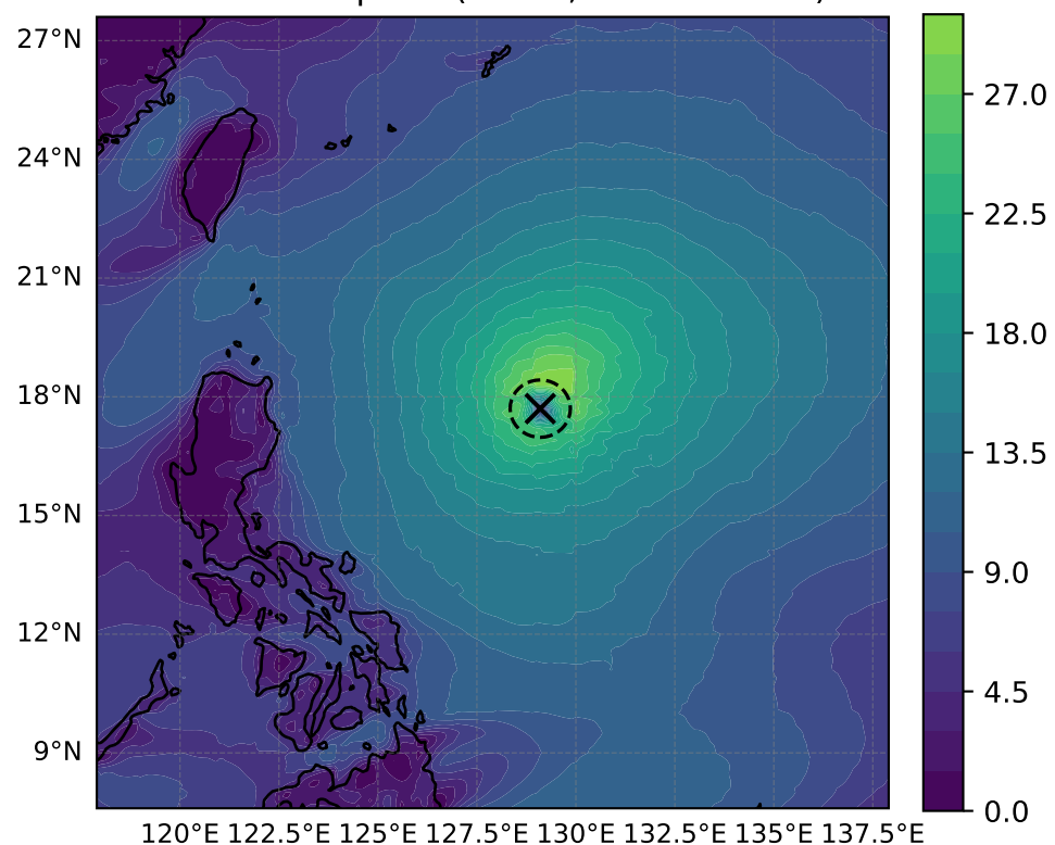
10 m windspeed ( \text{m s}^{-1} , max = 29.86)
