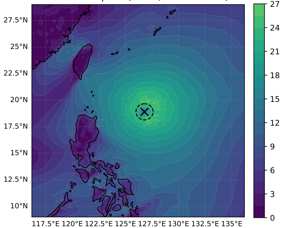
10 m windspeed ( \text{m s}^{-1} , max = 26.38)
