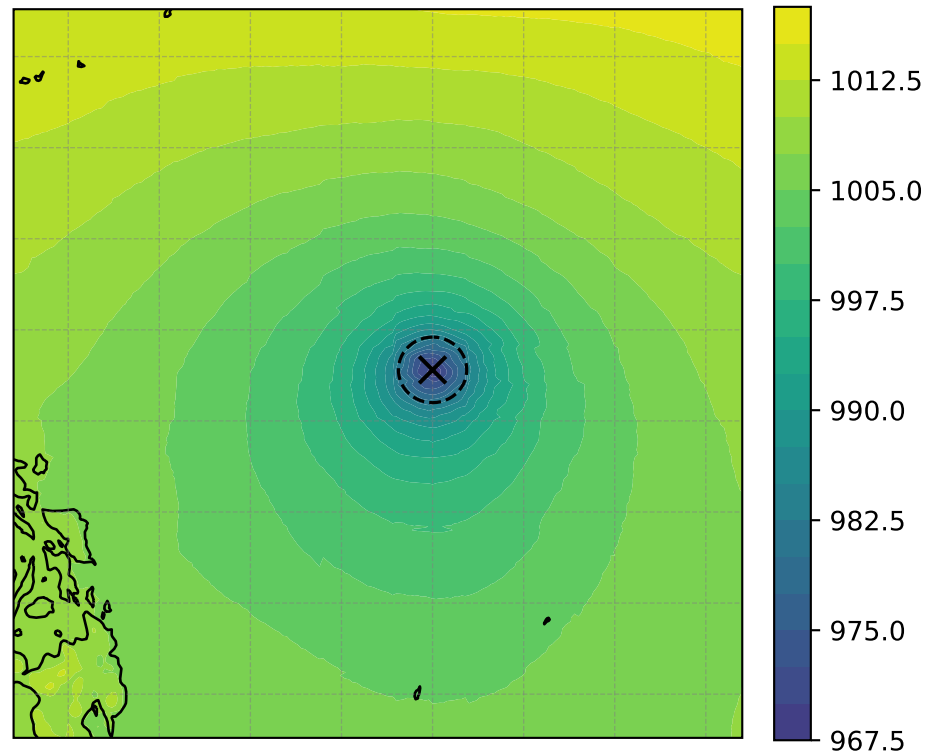
MSLP (hPa, min = 968.51)
