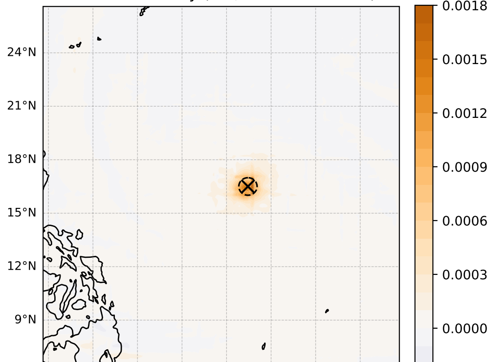
850 hPa vorticity ( \text{s}^{-1} , max = 1.78\text{e-}03 )
