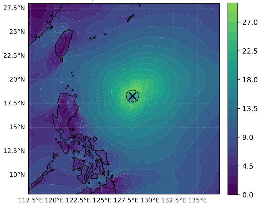
10 m windspeed ( \text{m s}^{-1} , max = 28.87)
