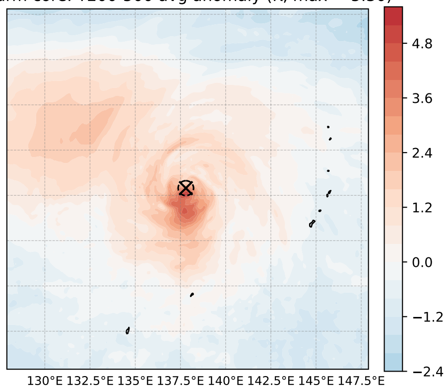
warm core: T200-500 avg anomaly (K, max = 5.30)
