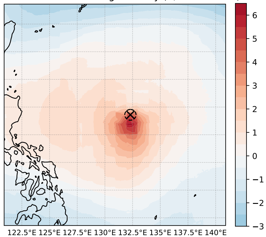
warm core: T200-500 avg anomaly (K, max = 6.24)
