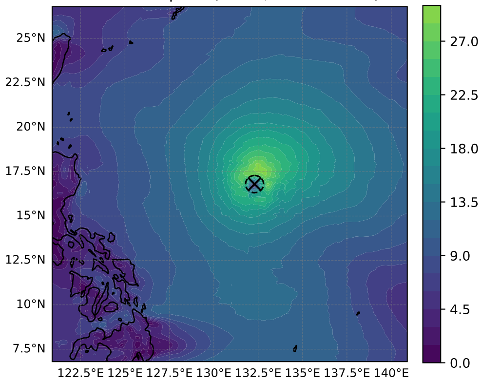
10 m windspeed ( \text{m s}^{-1} , max = 29.75)
