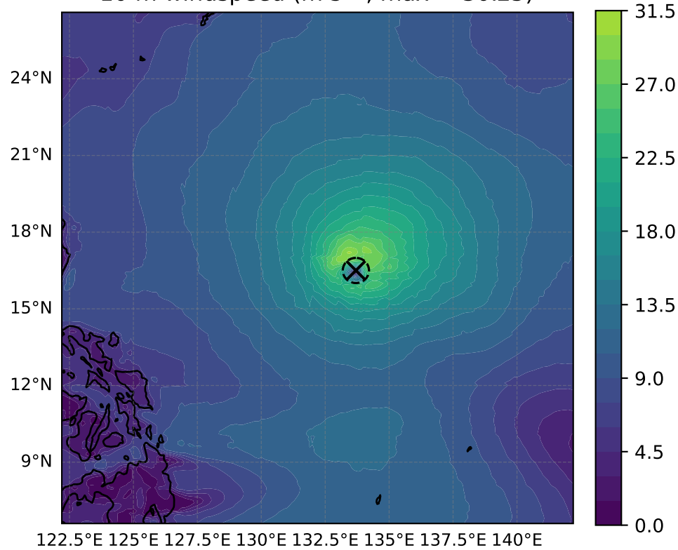
10 m windspeed ( \text{m s}^{-1} , max = 30.25)
