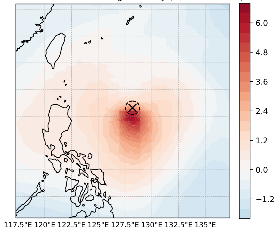
warm core: T200-500 avg anomaly (K, max = 6.54)
