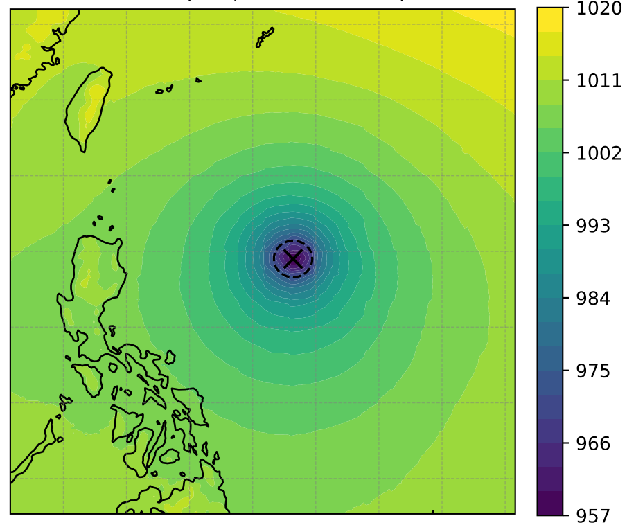
MSLP (hPa, min = 957.31)
