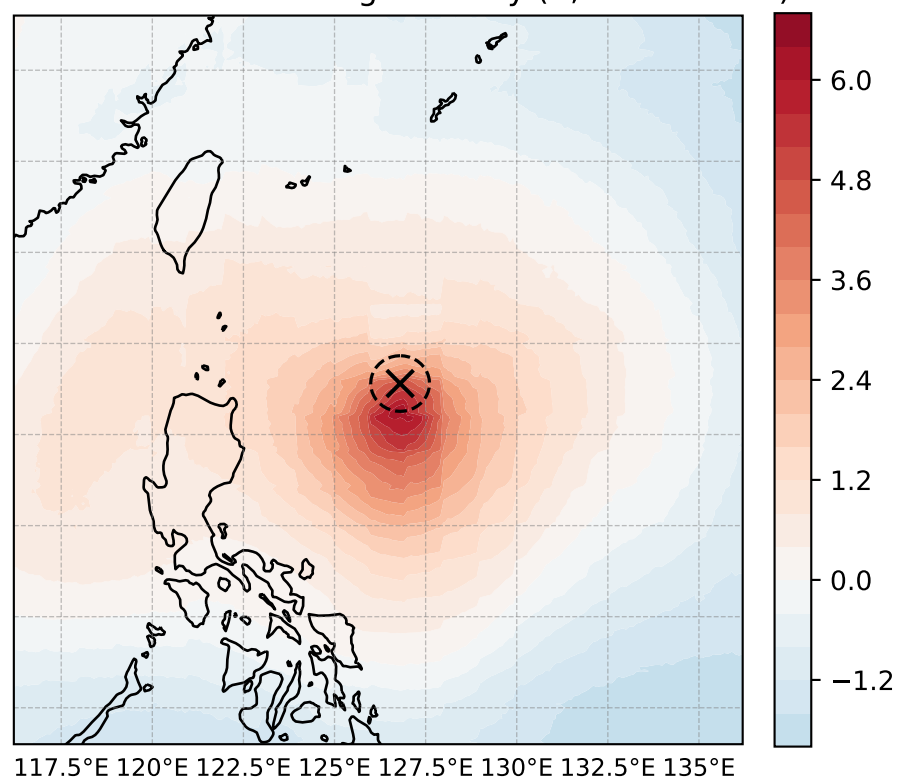
warm core: T200-500 avg anomaly (K, max = 6.50)
