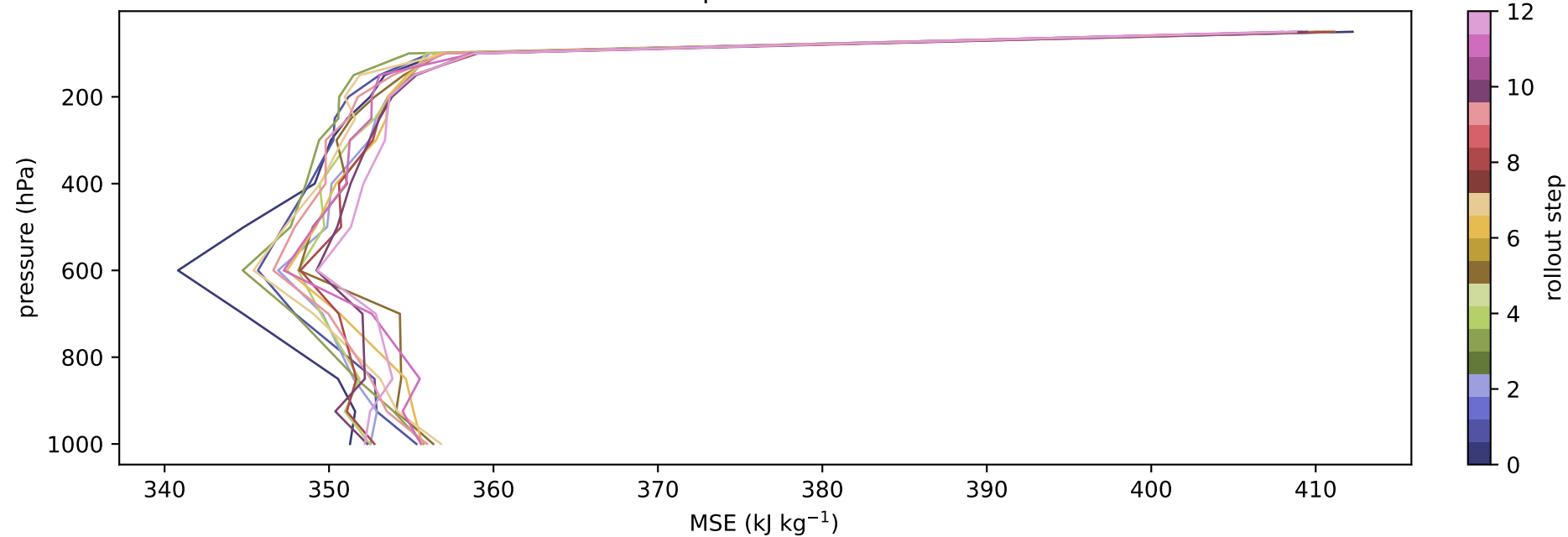
MSE vertical profile at storm centre
