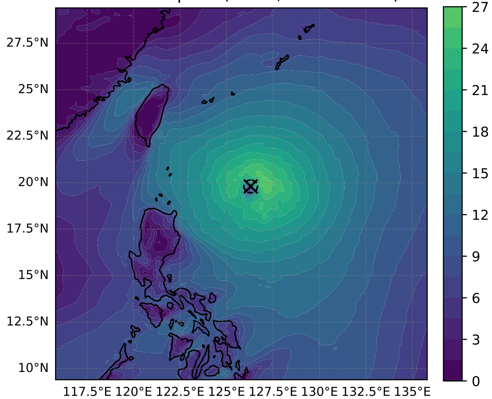
10 m windspeed ( \text{m s}^{-1} , max = 26.67)
