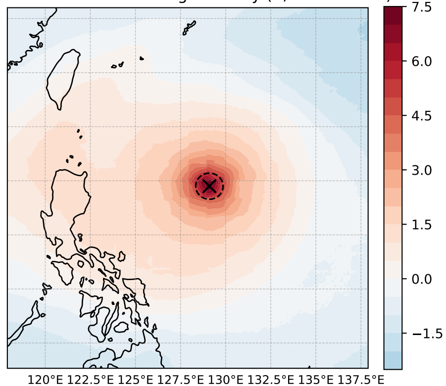
warm core: T200-500 avg anomaly (K, max = 7.50)
