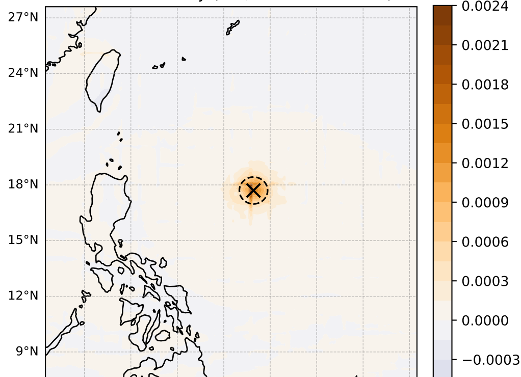
850 hPa vorticity ( \text{s}^{-1} , max = 2.26\text{e-}03 )
