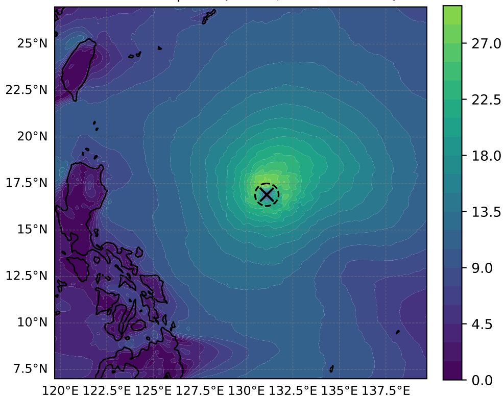
10 m windspeed ( \text{m s}^{-1} , max = 29.83)
