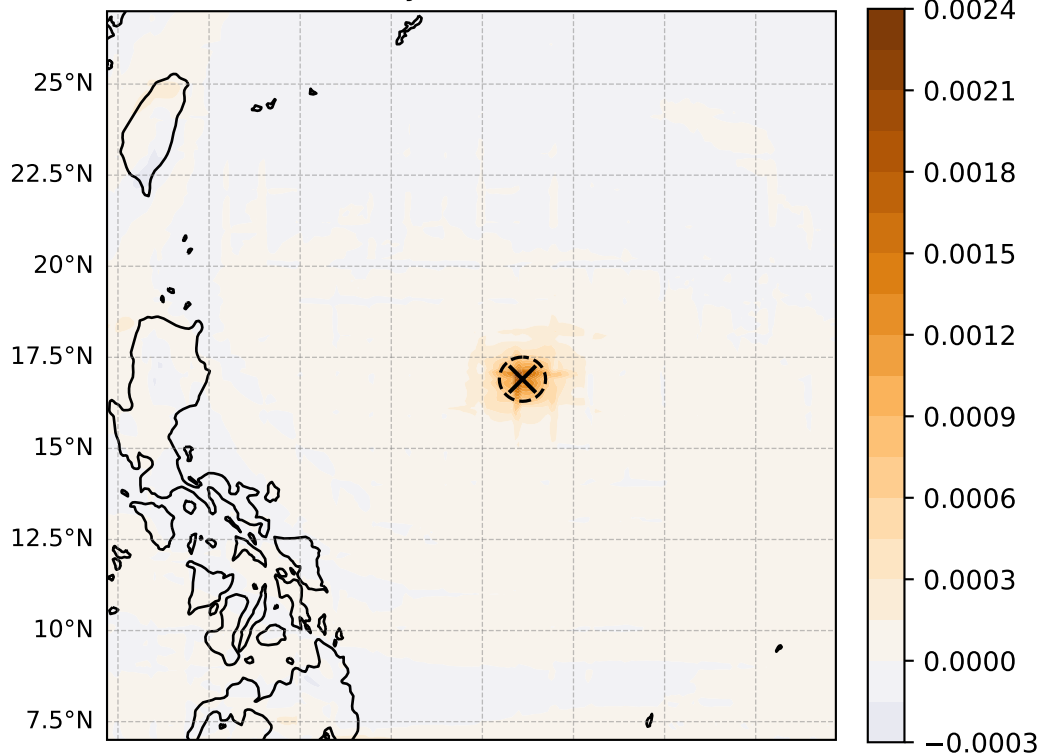
850 hPa vorticity ( \text{s}^{-1} , max = 2.32\text{e-}03 )
