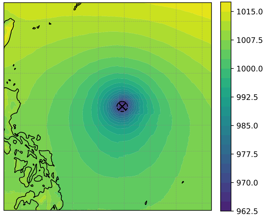
MSLP (hPa, min = 964.81)
