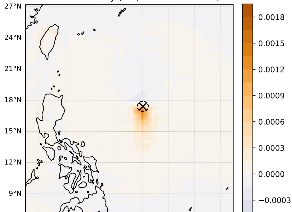
850 hPa vorticity ( \text{s}^{-1} , max = 1.94\text{e-}03 )
