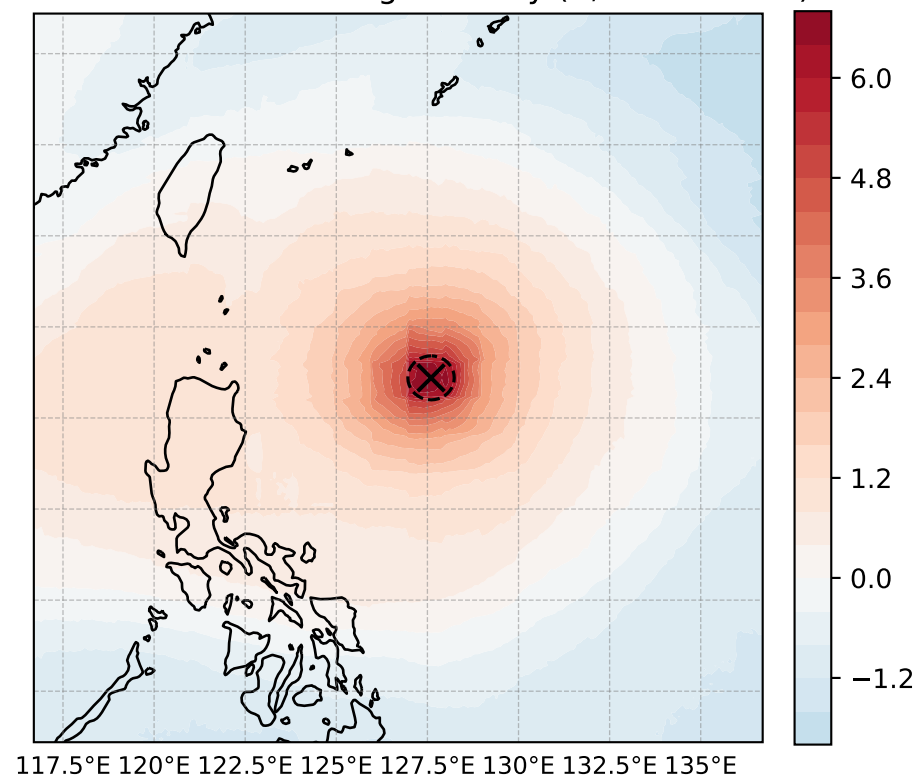
warm core: T200-500 avg anomaly (K, max = 6.73)
