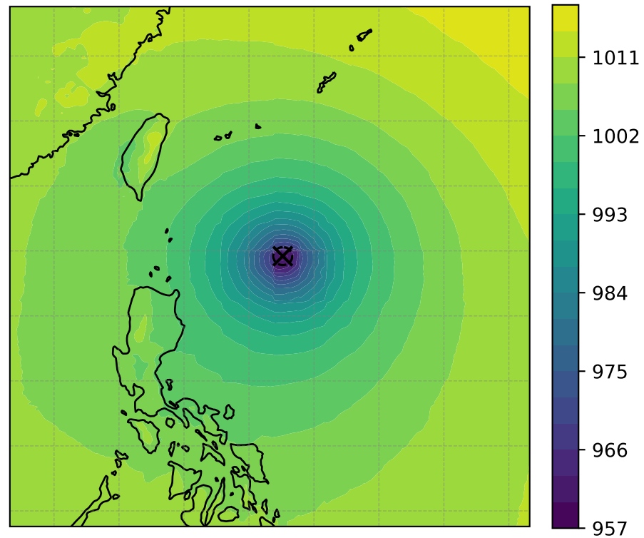
MSLP (hPa, min = 959.25)
